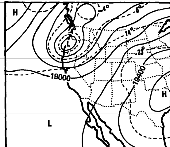
Figure 2.10.--500-mb charts for August 26-29, 1951.
