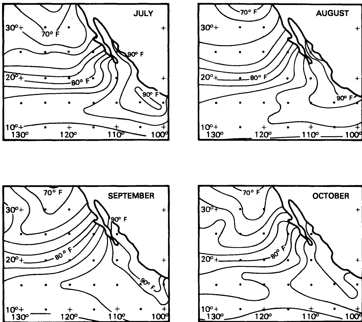
Figure 2.46.--Maximum sea-surface temperature charts for the tropical Pacific for July, August, September and October (Laviolette and Seim 1969).
