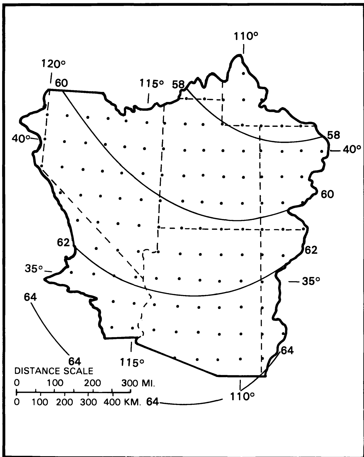
Figure 4.30.--1000-mb 12-hr persisting general dew point for mid-November.
