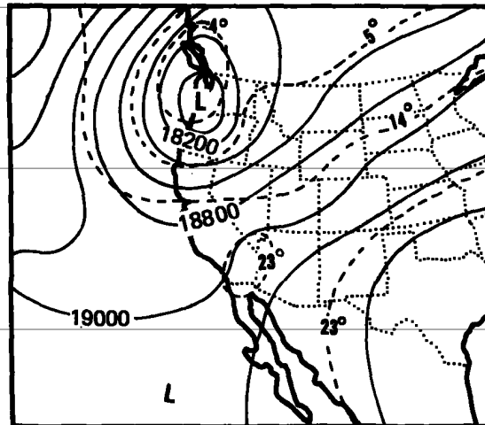
Figure 2.10.--500-mb charts for August 26-29, 1951.
