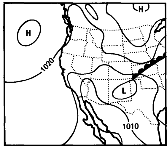
Figure 2.35b.--Surface weather map for June 6, 1943.
