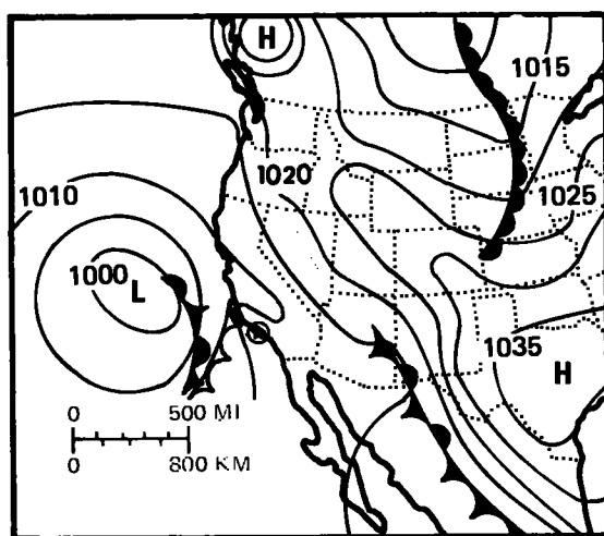
Figure 3.40.--Surface weather maps for March 3-4, 1934.
