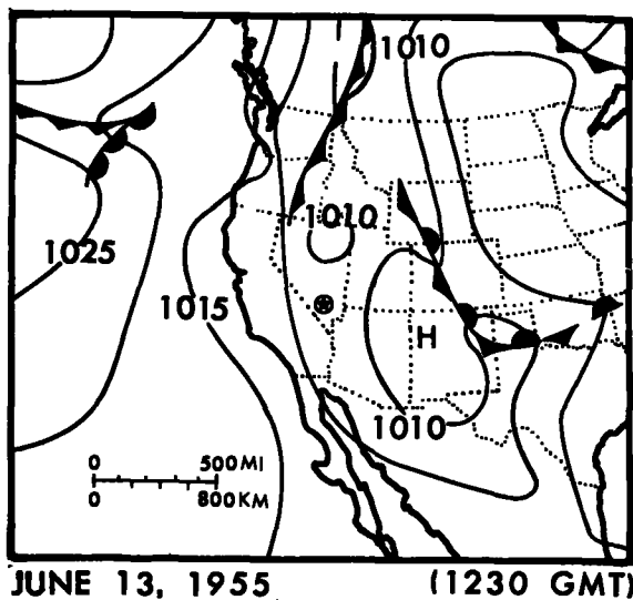
Figure 3.21. Surface weather maps for June 13-14, 1955.
