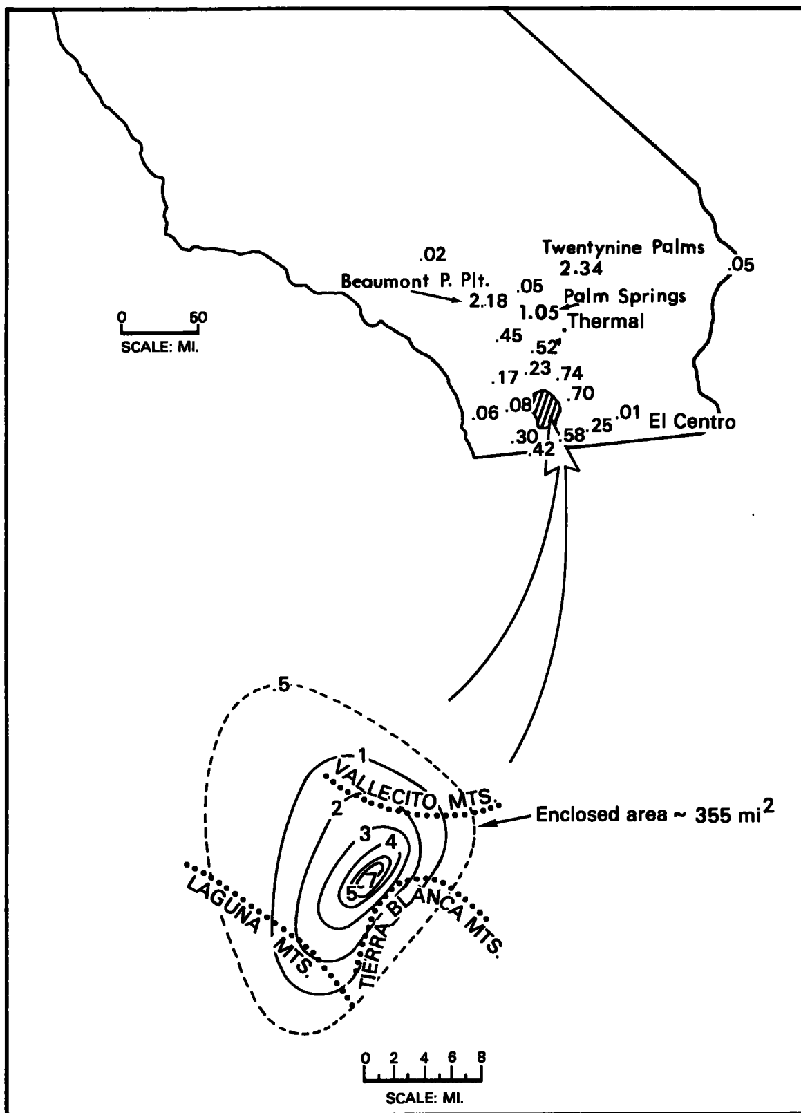
Figure 3.12.--Isohyetal map for storm at Vallecito, Calif. on July 18, 1955. Rainfall data are shown for other stations in southern California.
