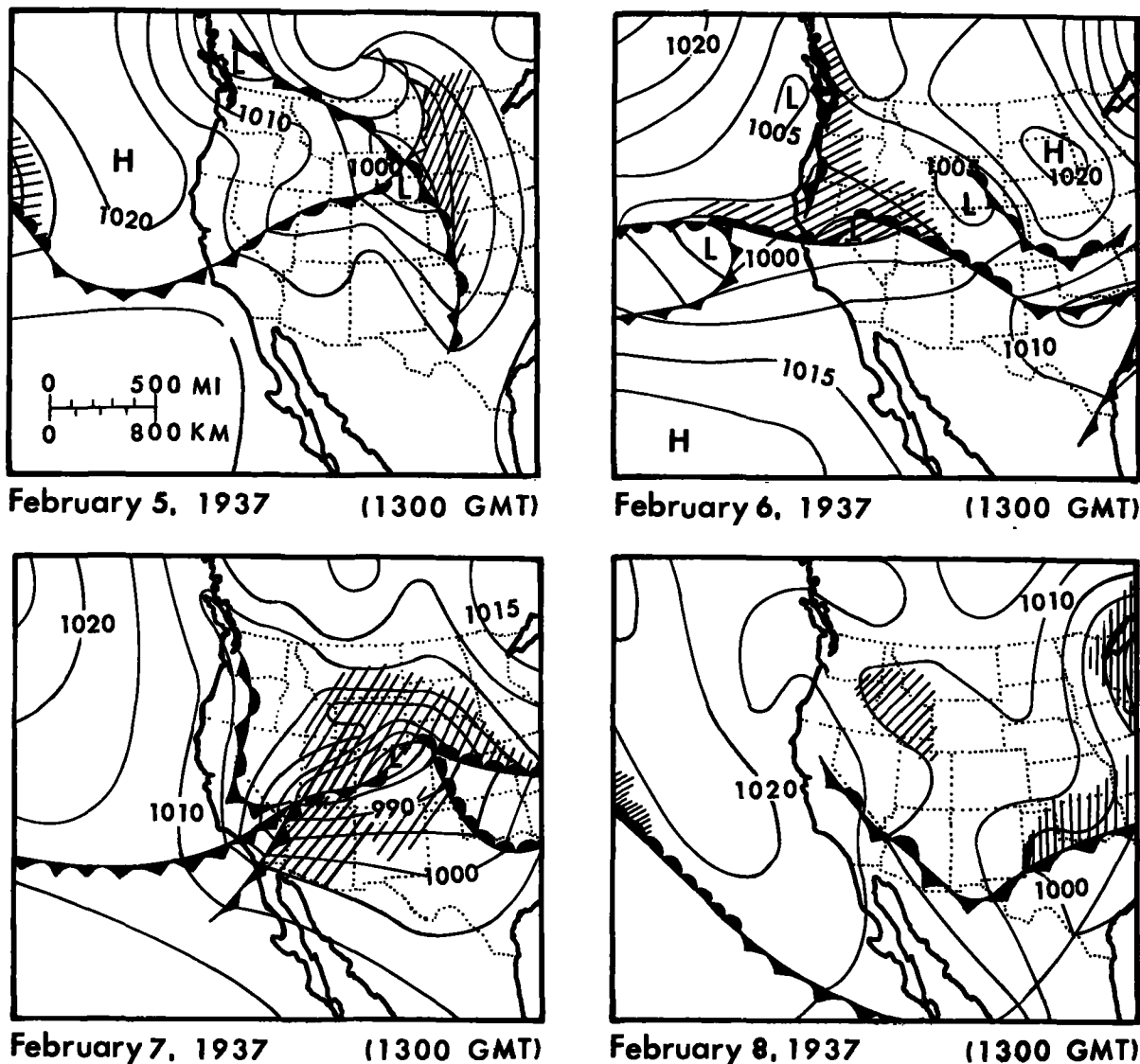
Figure 2.37.--Surface weather maps for February 5-8, 1937.
