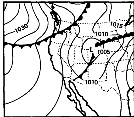
Figure 2.25.--Surface weather maps for October 26-29, 1946.
