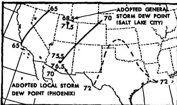
A--ANALYSIS OF MAXIMUM OBSERVED PRECIPITABLE WATER EXPRESSED AS 1000-MB DEW POINTS (°F)
