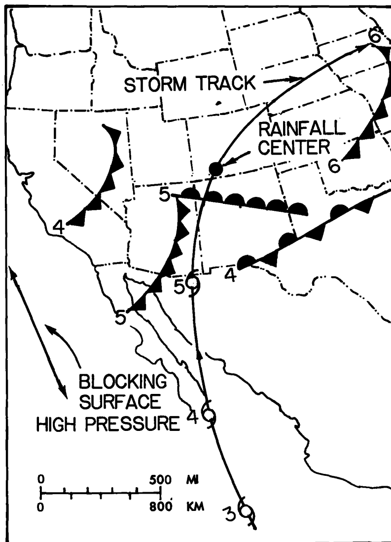
Figure 2.19.--Storm track and significant weather features for storm of October 4-6, 1911.
