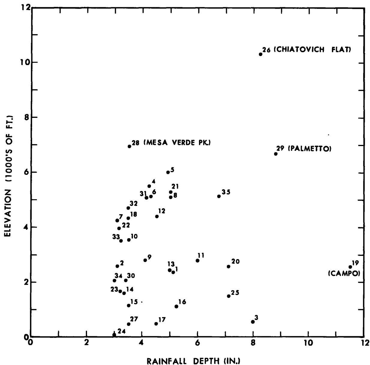
Figure 3.2.--Point rainfall extremes for local storms vs. elevation at which the data were observed. Refer to table 3.1 for storm identification.
