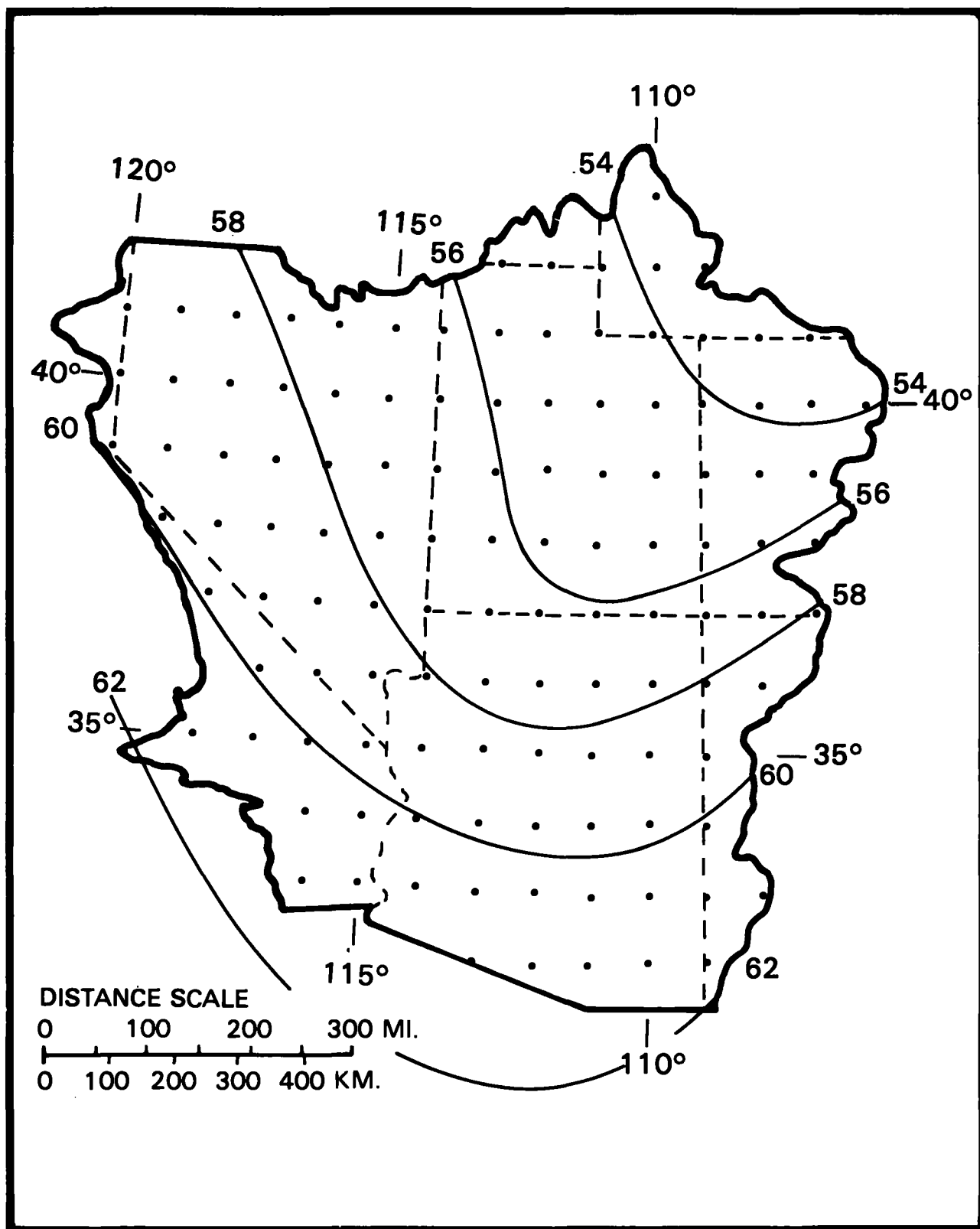
Figure 4.31.--1000-mb 12-hr persisting dew point for mid December.
