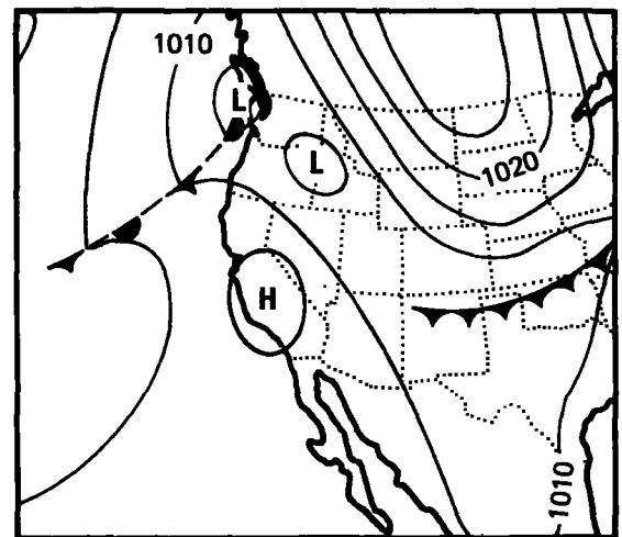
Figure 2.17.--Surface weather maps for October 4-6, 1925 and schematic diagram showing estimated upper level trough positions.
