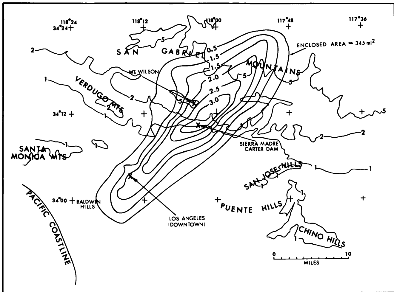
Figure 3.39.--Isohyetal map for storm of March 3, 1943.
