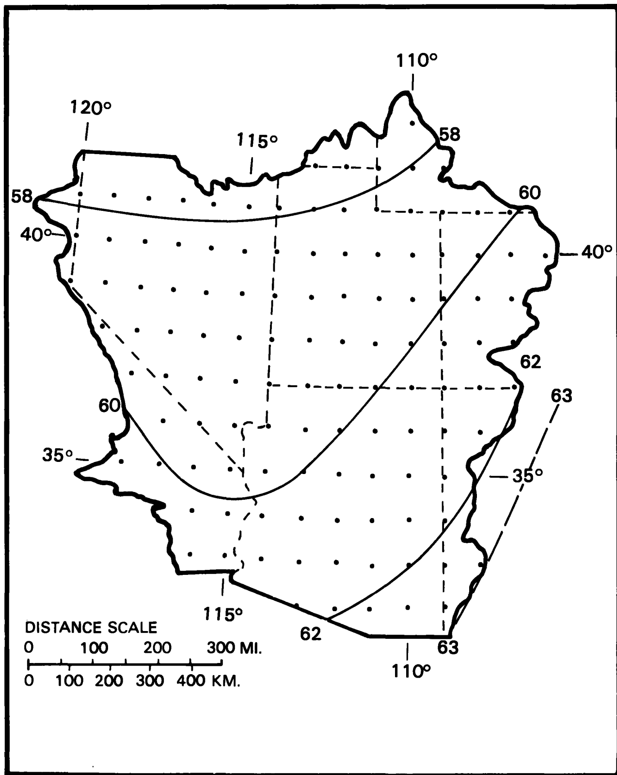
Figure 4.17.--1000-mb 12-hr persisting general storm dew point for mid-April.
