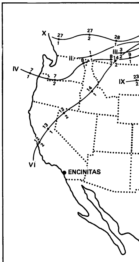
Figure 3.30.--Storm tracks for October 1889.
