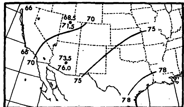
B--MAXIMUM PERSISTING 12-HR 1000-MB DEW POINTS (°F). AFTER ENVIRONMENTAL DATA SERVICE (1968)
