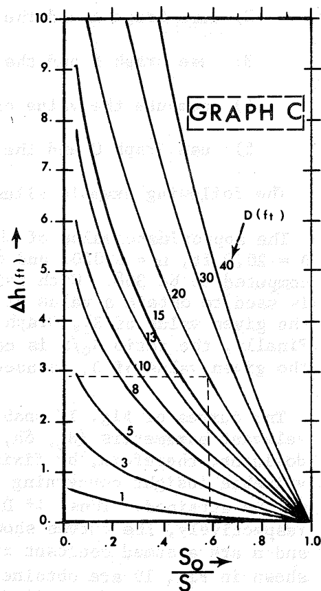
Figure 17. Generalized Graphical Estimation of Magnitude ( \Delta h ) of the Dynamic Loop.
