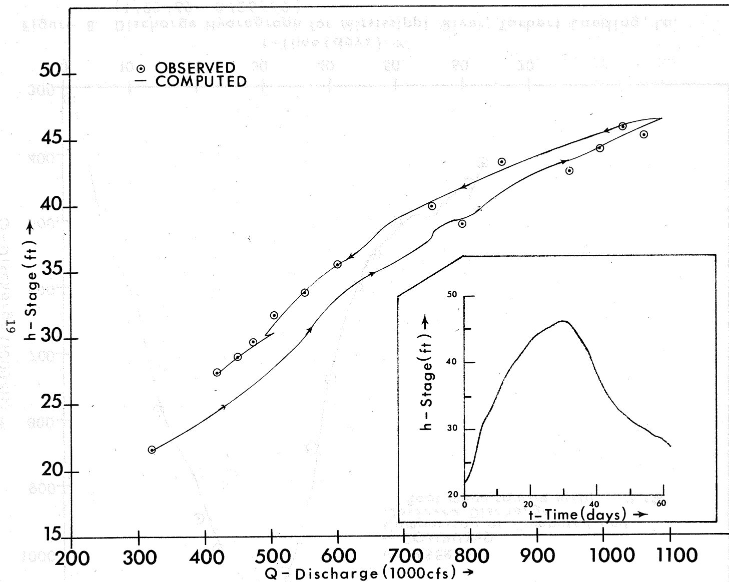
Figure 7. Stage-Discharge Relation for Mississippi River, Tarbert Landing, La. (1/23/69 - 3/26/69).
