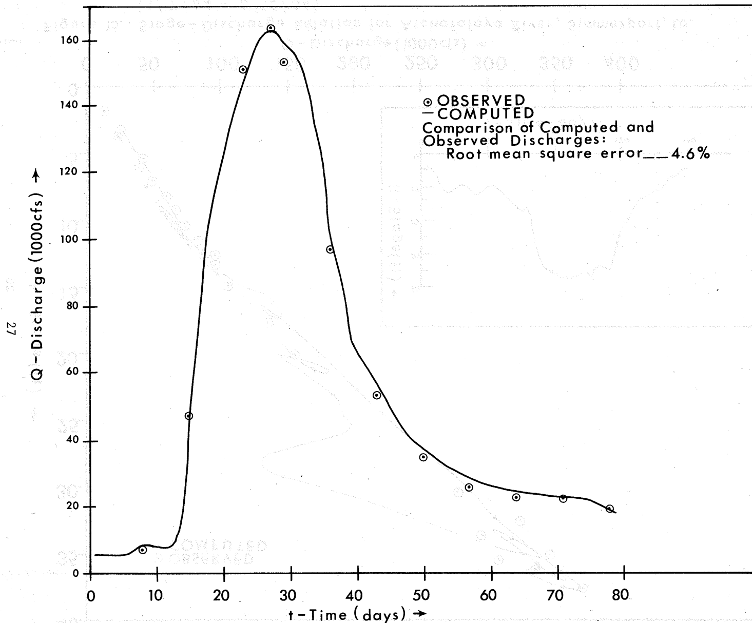
Figure 14. Discharge Hydrograph for Red River, Alexandria, La. (4/13/66-7/1/66).
