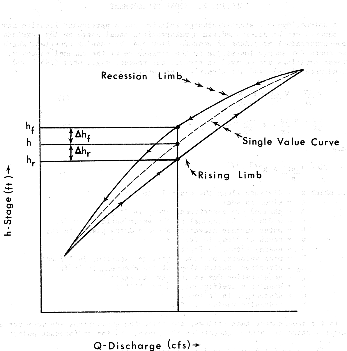
Figure 2. Stage - Discharge Relation with Hysteresis Loop Due to Changing Discharge.
