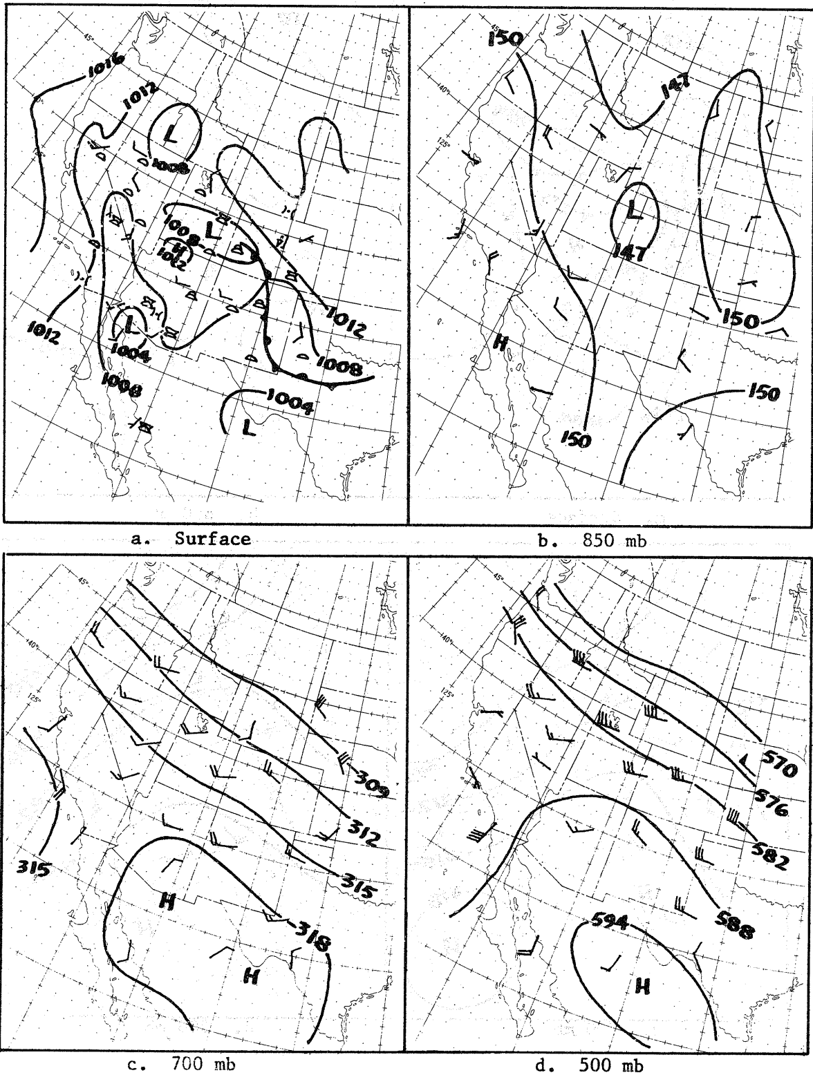
Figure 3.--Standard pressure level charts for June 21, 1972, 0000 GMT. Pressure in millibars, heights in decameters, winds in knots.
