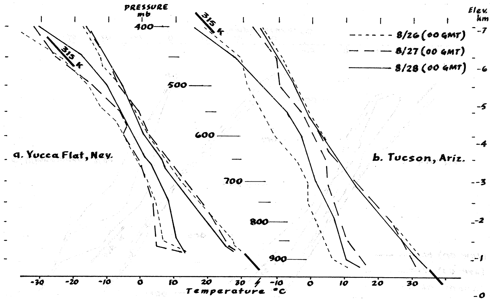
Figure 12.--Temperature and dew-point soundings for August 26-28, 1970. Slope of 315K isotherm represents dry adiabatic lapse rate.
