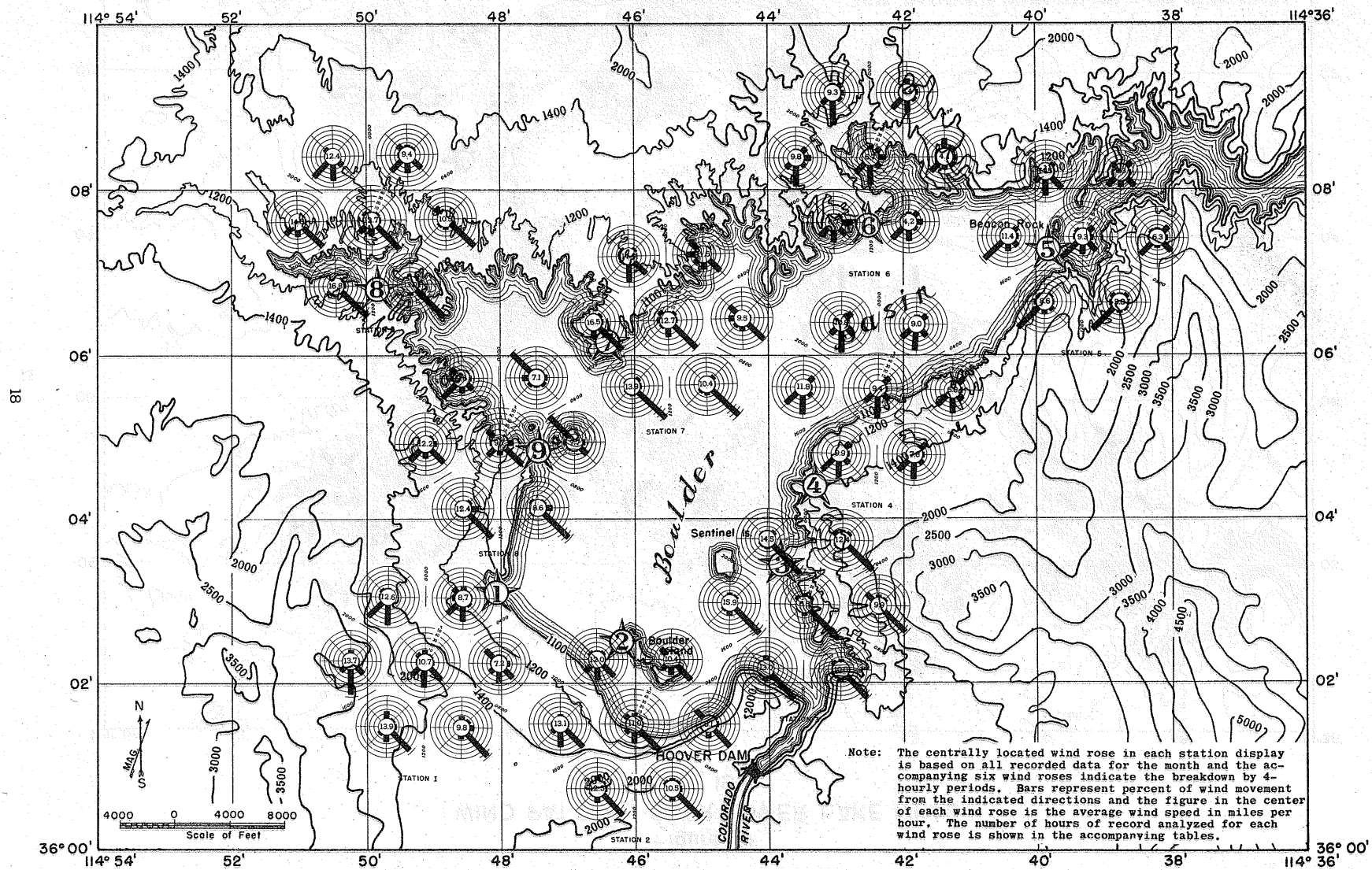
Figure 15 WIND PATTERN OVER LOWER LAKE MEAD JUNE, 1951
