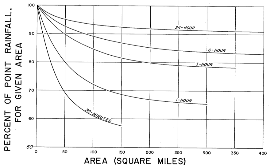
AREA-DEPTH CURVES
