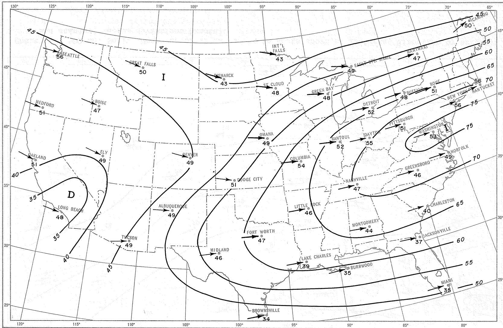
Chart 5. - 300 mb. Winter. Mean vector winds (speed in knots shown by isotachs, direction by arrows) and standard vector deviations (knots).
