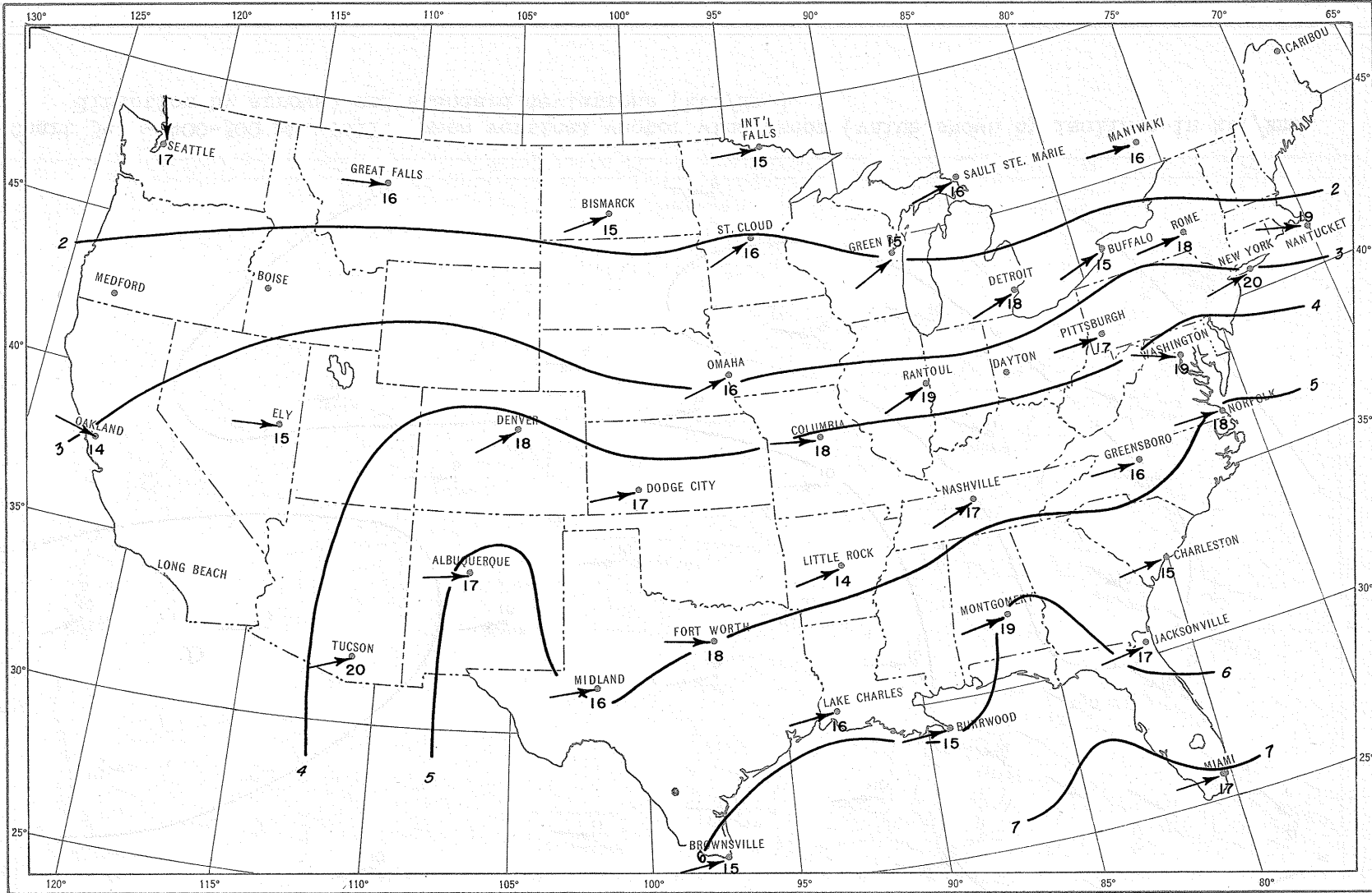
Chart 35. - 300-250 mb. Winter. Mean vertical vector wind shear (value shown by isolines in kt./km., direction by arrows) and standard deviations (kt./km.).
