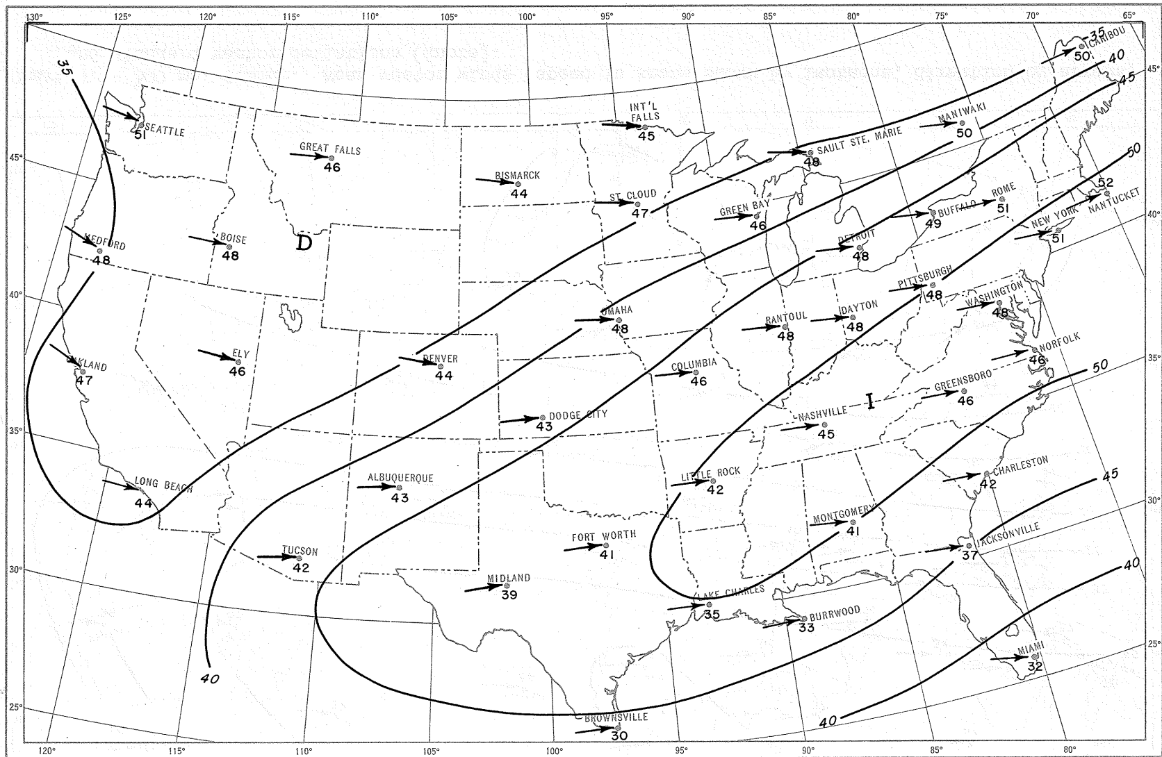
Chart 6. - 300 mb. Spring. Mean vector winds (speed in knots shown by isotachs, direction by arrows) and standard vector deviations (knots).
