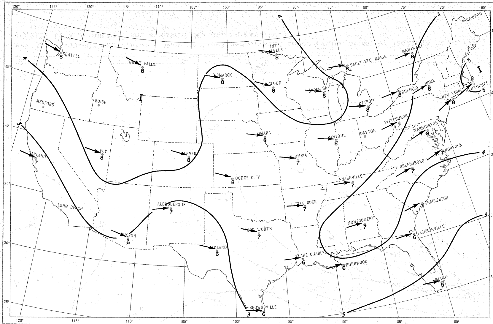
Chart 30. - 700-500 mb. Fall. Mean vertical vector wind shear (value shown by isolines in kt./km., direction by arrows) and standard deviations (kt./km.).
