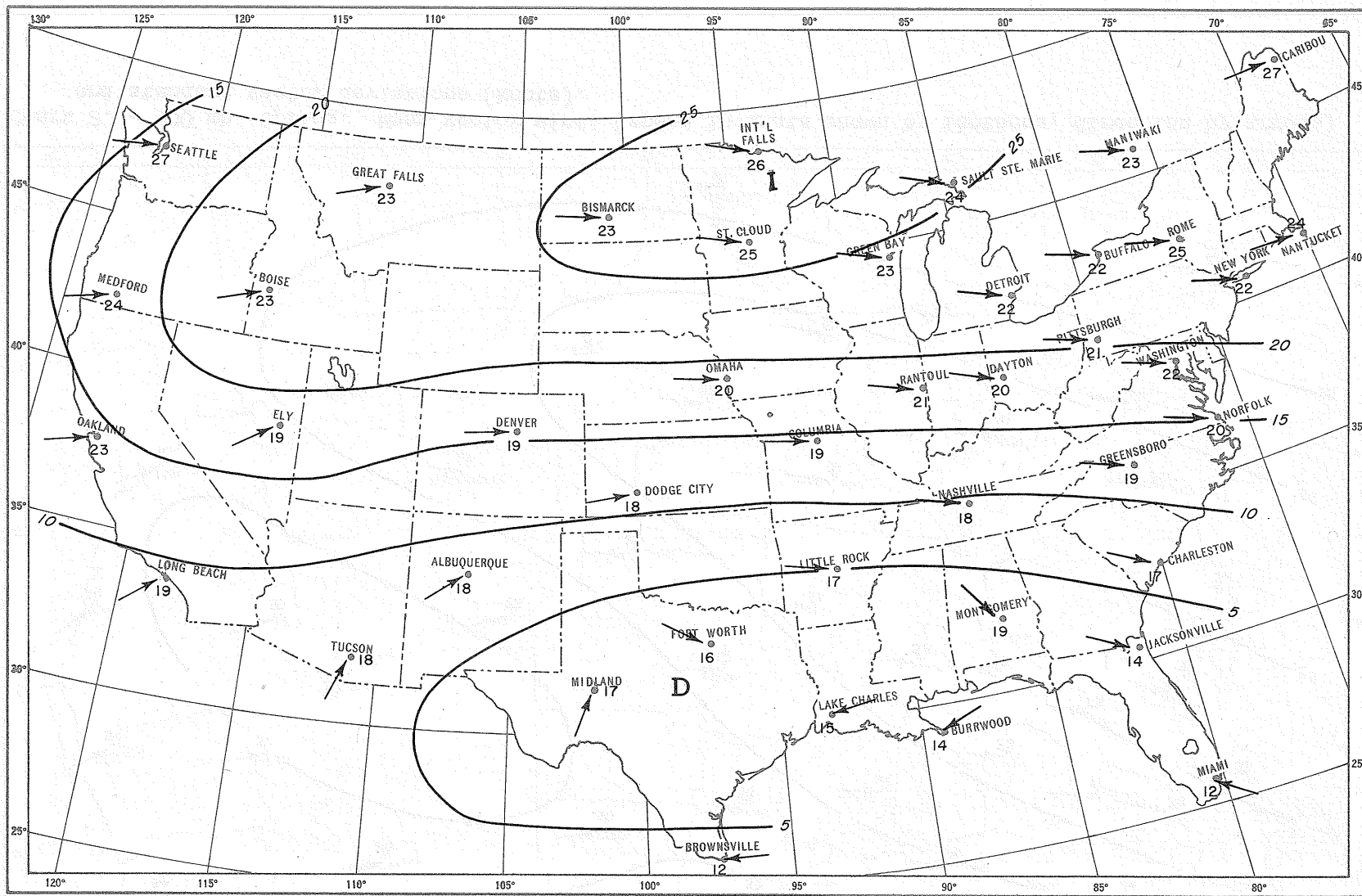
Chart 3. - 500 mb. Summer. Mean vector winds (speed in knots shown by isotachs, direction by arrows) and standard vector deviations (knots).
