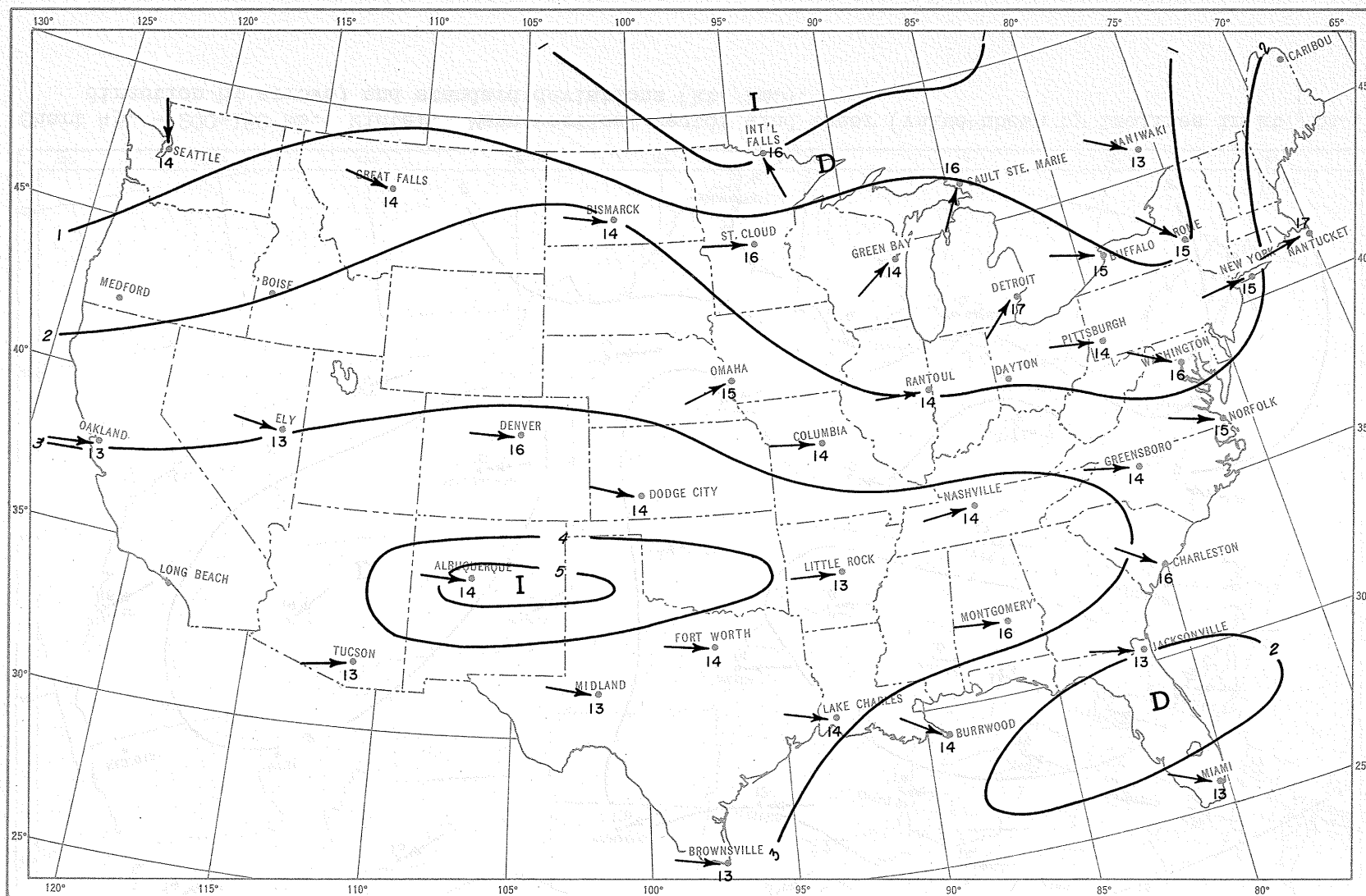
Chart 42. - 250-200 mb. Fall. Mean vertical vector wind shear (value shown by isolines in kt./km., direction by arrows) and standard deviations (kt./km.).
