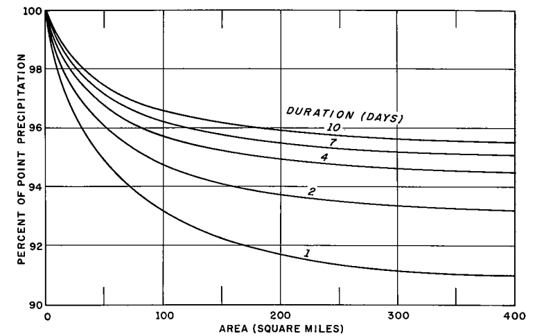
FIGURE 10.—Depth-area curves.
