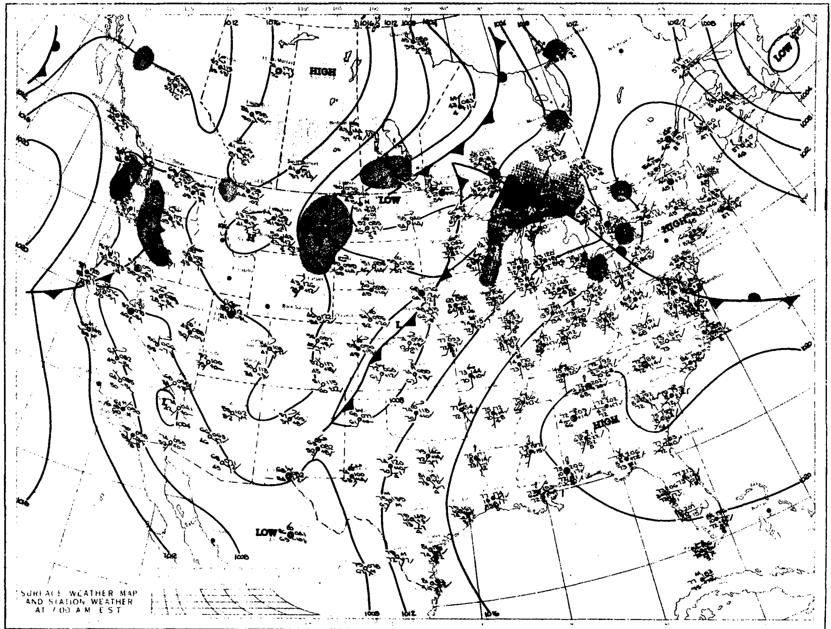
Figure 7-9.--Surface weather analysis at 0600 CST, August 16, 1968.
