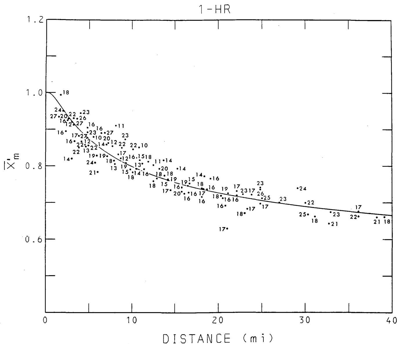
Figure 2-2.--Relative mean of annual series of two-station averages, 1-hr vs. interstation distance. Points identified with direction between stations. Same data as figure 3-1.
