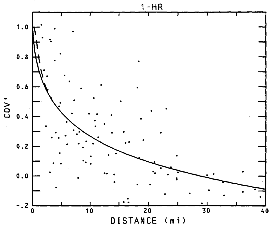
Figure 4-14.--Variation with interstation distance of relative covariance of maximum annual point rainfall and simultaneous rain at a second point, \text{cov}'_{Ab} , 1-hr.
