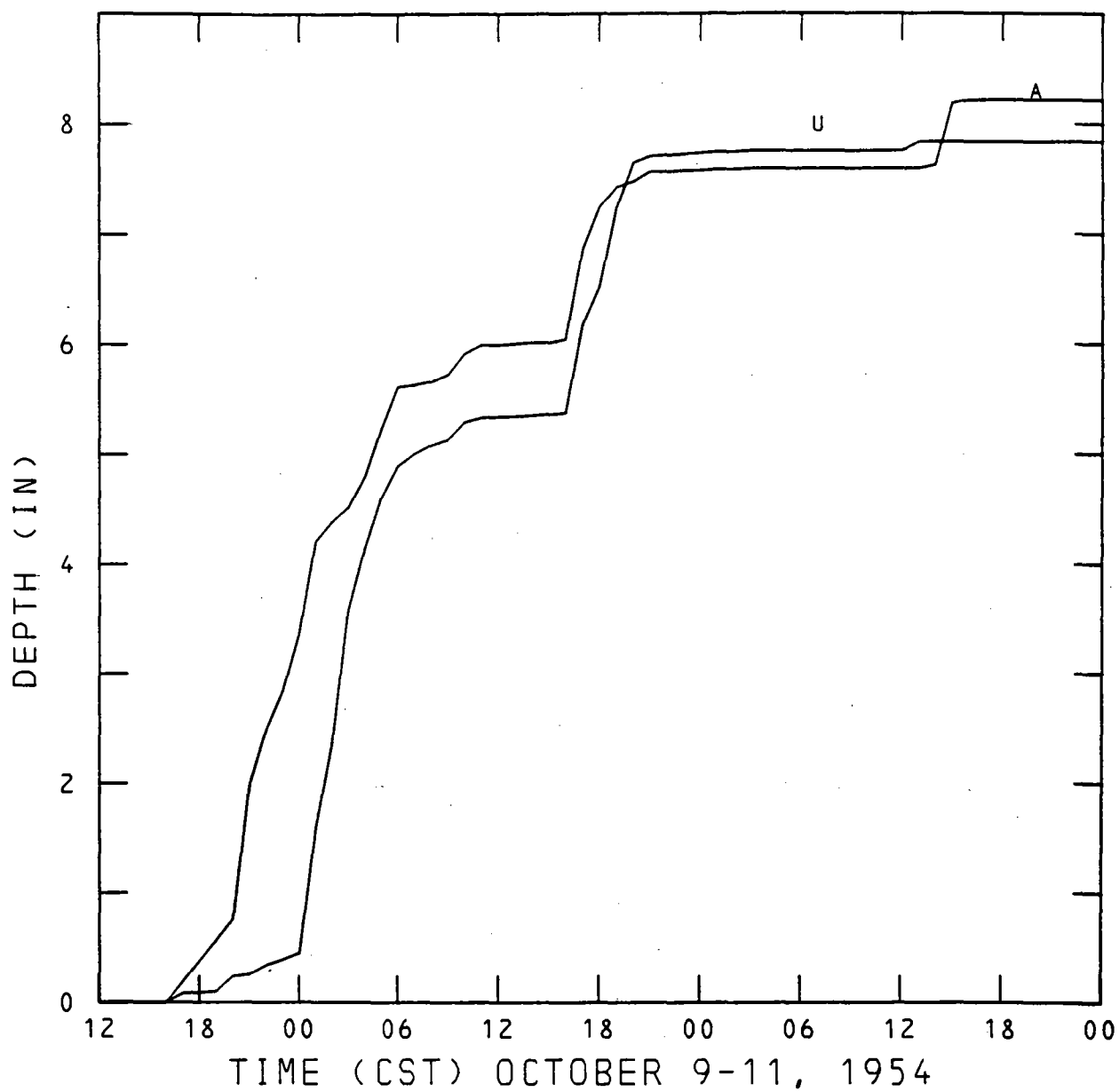
Figure 7-4.--Precipitation mass curves for Chicago Calumet Treatment Works (Station A) and Crete (Station U), October 9-11, 1954.
