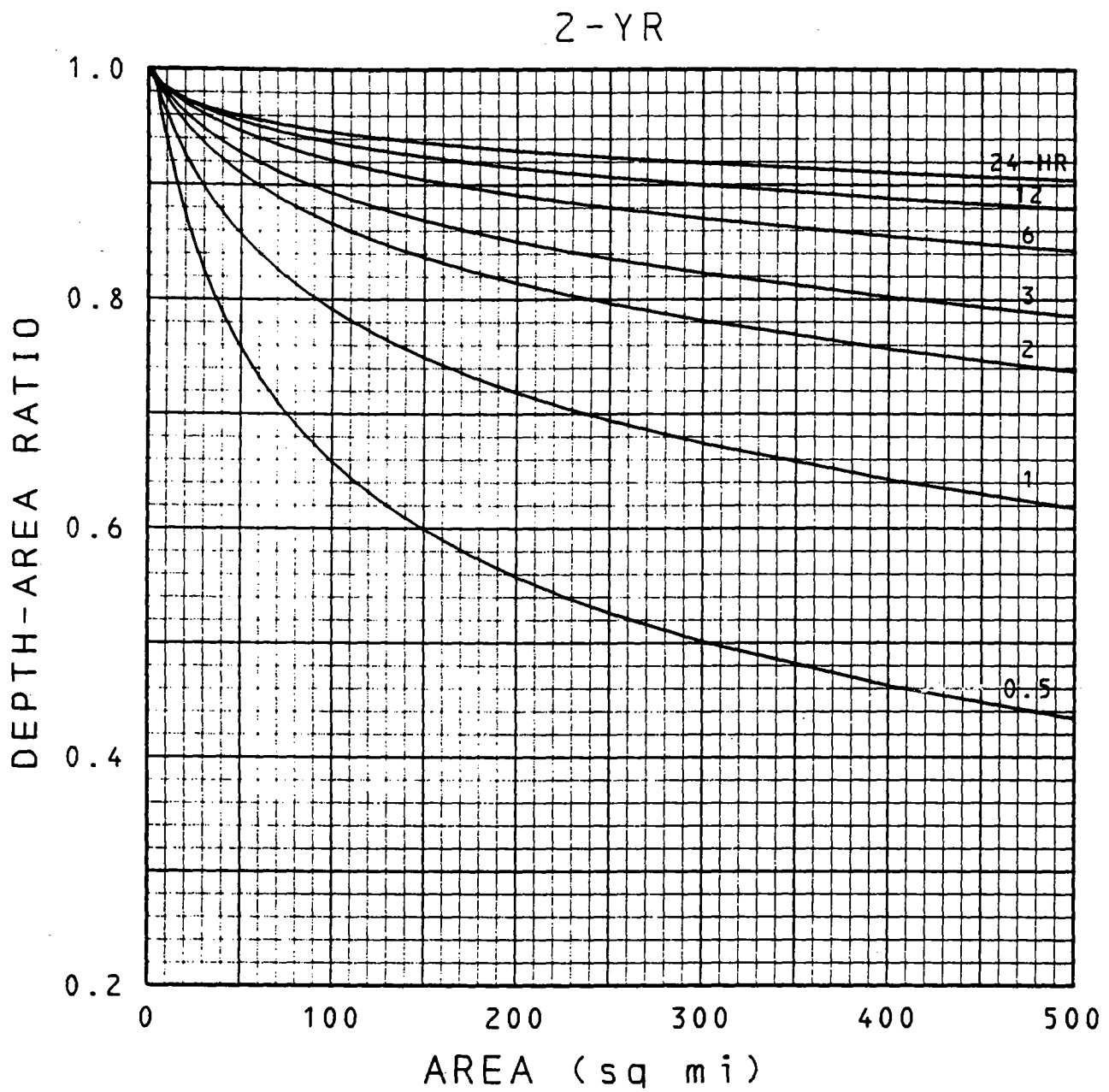
Figure 6-1.--Depth-area ratios. Chicago, Ill. Areal profiles to 500 mi 2 , by duration, 2-yr.
