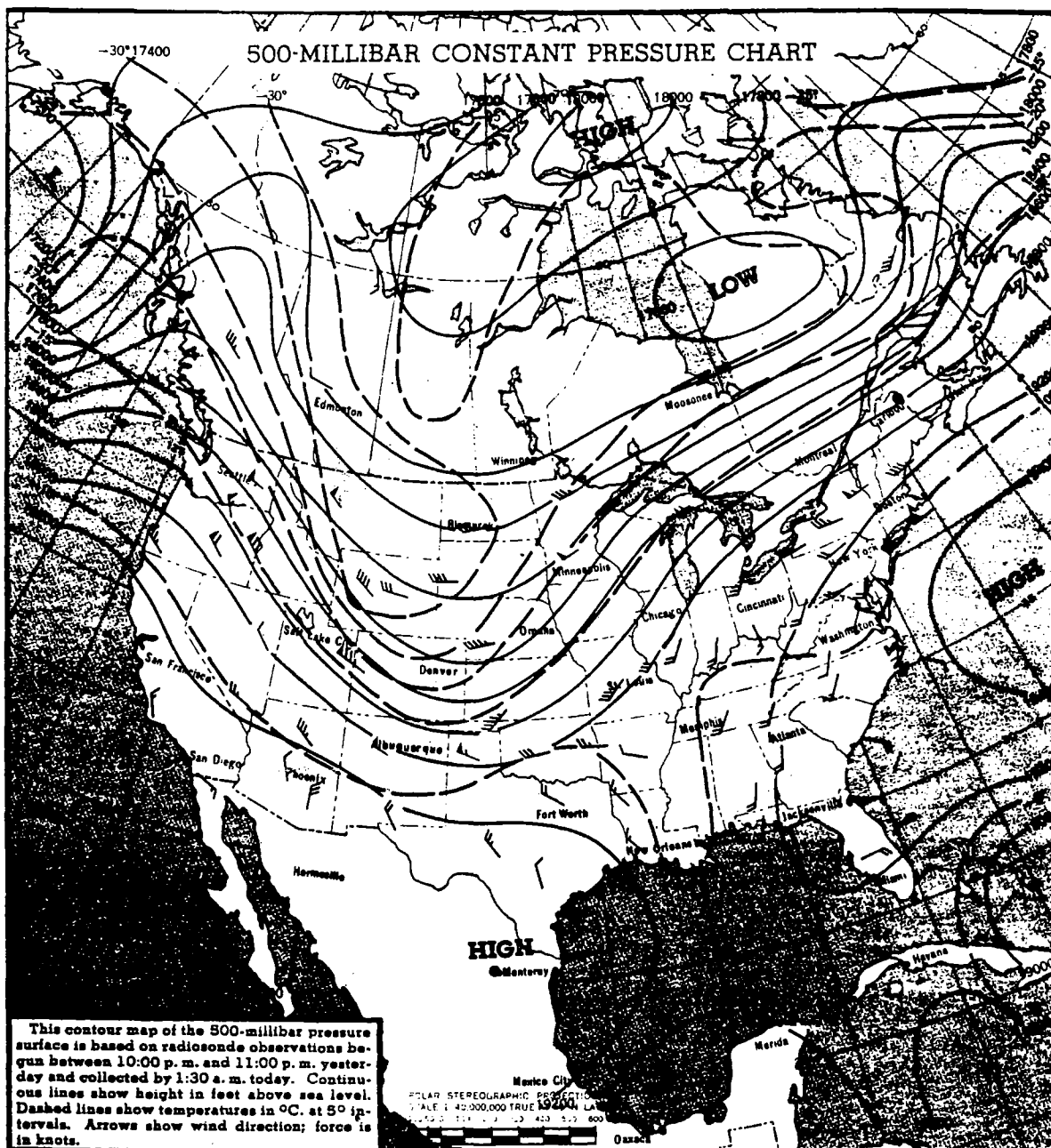
Figure 7-8.--500-mb analysis at 2200 CST, October 13, 1954.
