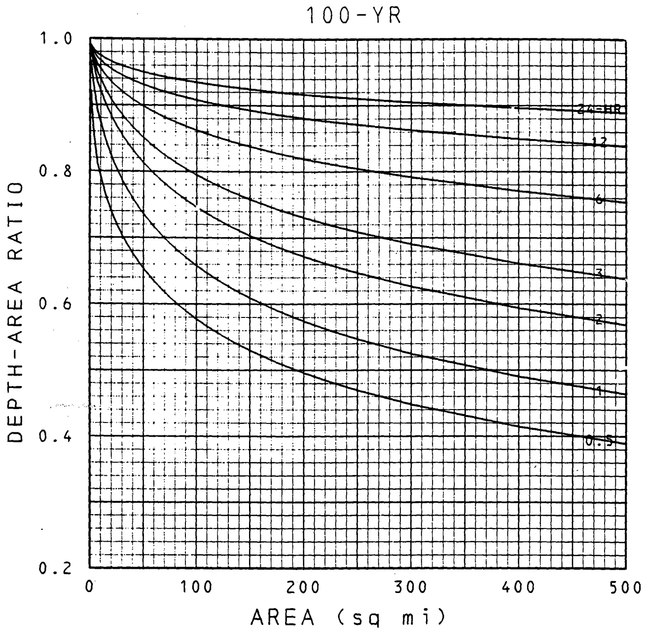
Figure 6-2.--Same as figure 6-1, 100-yr.
