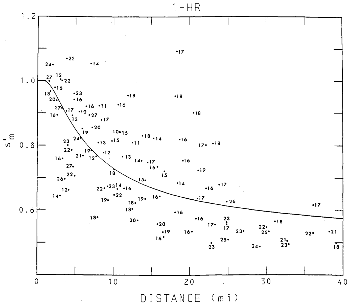
Figure 2-3.--Relative standard deviation of annual series of two-station averages, 1-hr vs. interstation distance. Points identified with direction between stations. Same data as figure 3-4.
