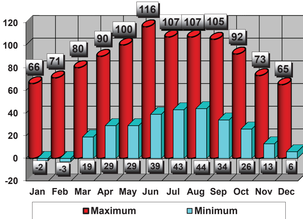
Portland Airport: Monthly Extremes (Oct 1940 through March 2022)
