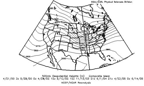
(h) Deep Progressive Midwest Trough (8 cases)
