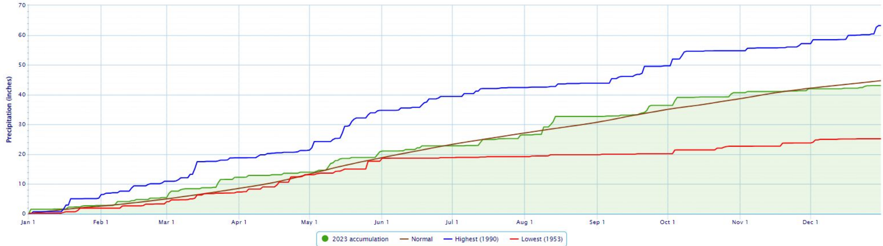
Accumulated Precipitation – SPRINGFIELD WSO AP, MO
