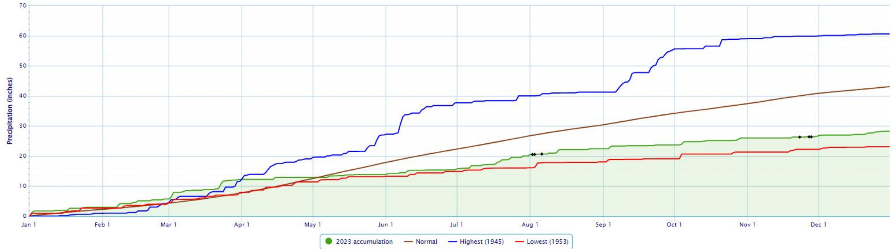
Accumulated Precipitation – VICHY ROLLA NATL AP, MO
