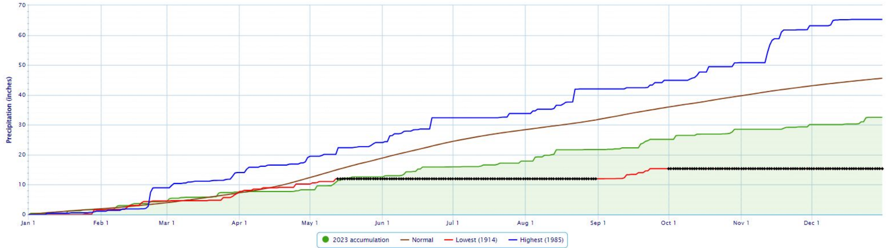
Accumulated Precipitation – JOPLIN REGIONAL AIRPORT, MO
