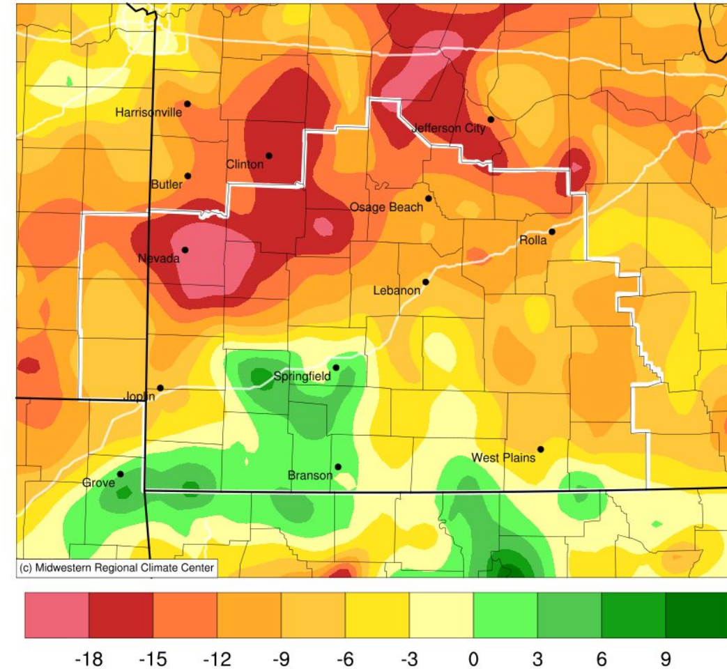
Accumulated Precipitation (in): Departure from 1991-2020 Normals January 01, 2023 to December 31, 2023
