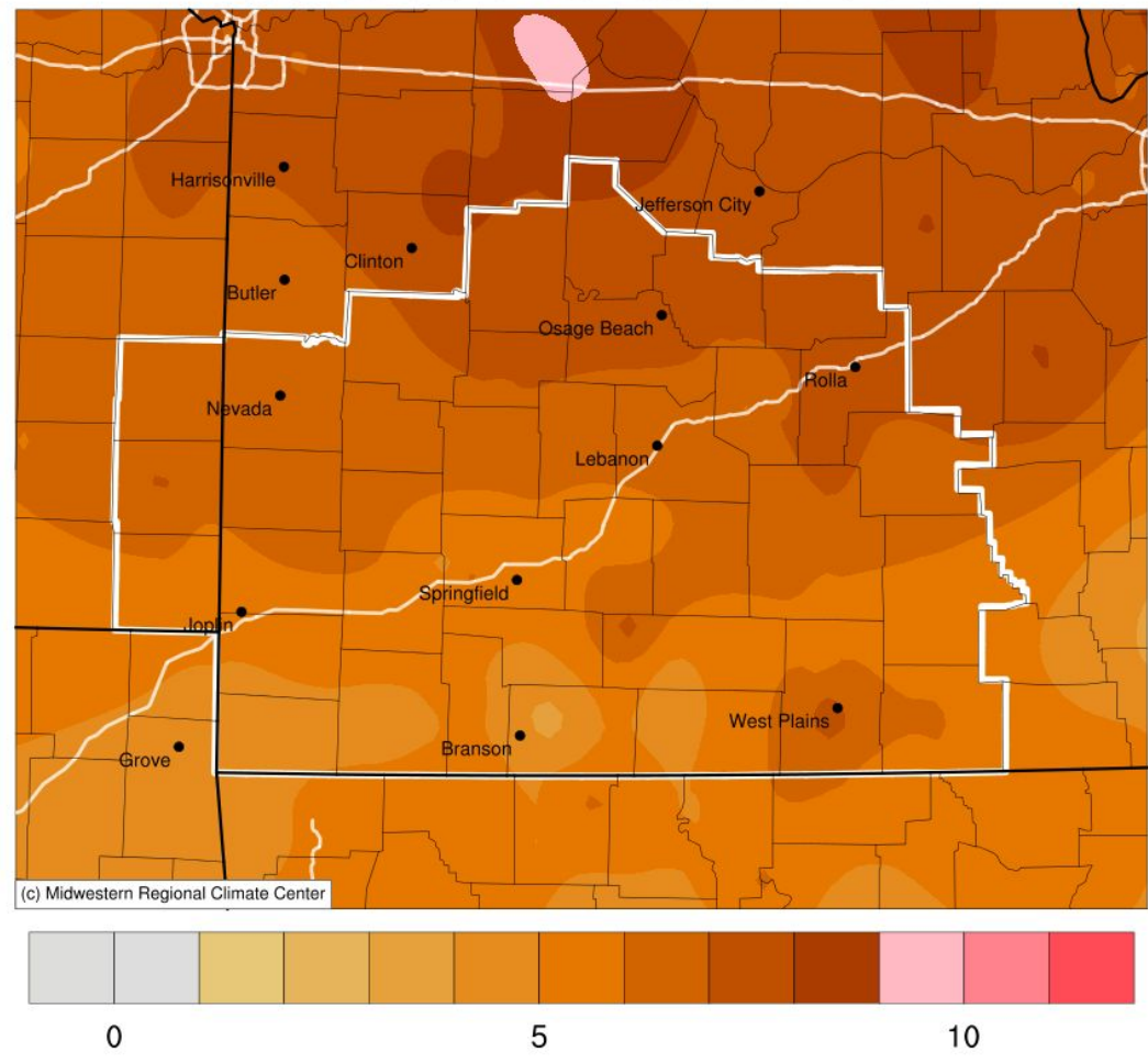
Average Temperature (°F): Departure from 1991-2020 Normals December 01, 2023 to December 31, 2023
