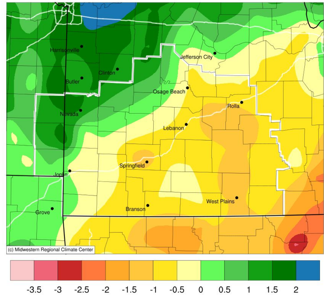
Accumulated Precipitation (in): Departure from 1991-2020 Normals December 01, 2023 to December 31, 2023
