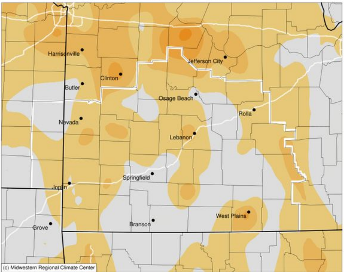
Average Temperature (°F): Departure from 1991-2020 Normals May 01, 2023 to May 31, 2023
