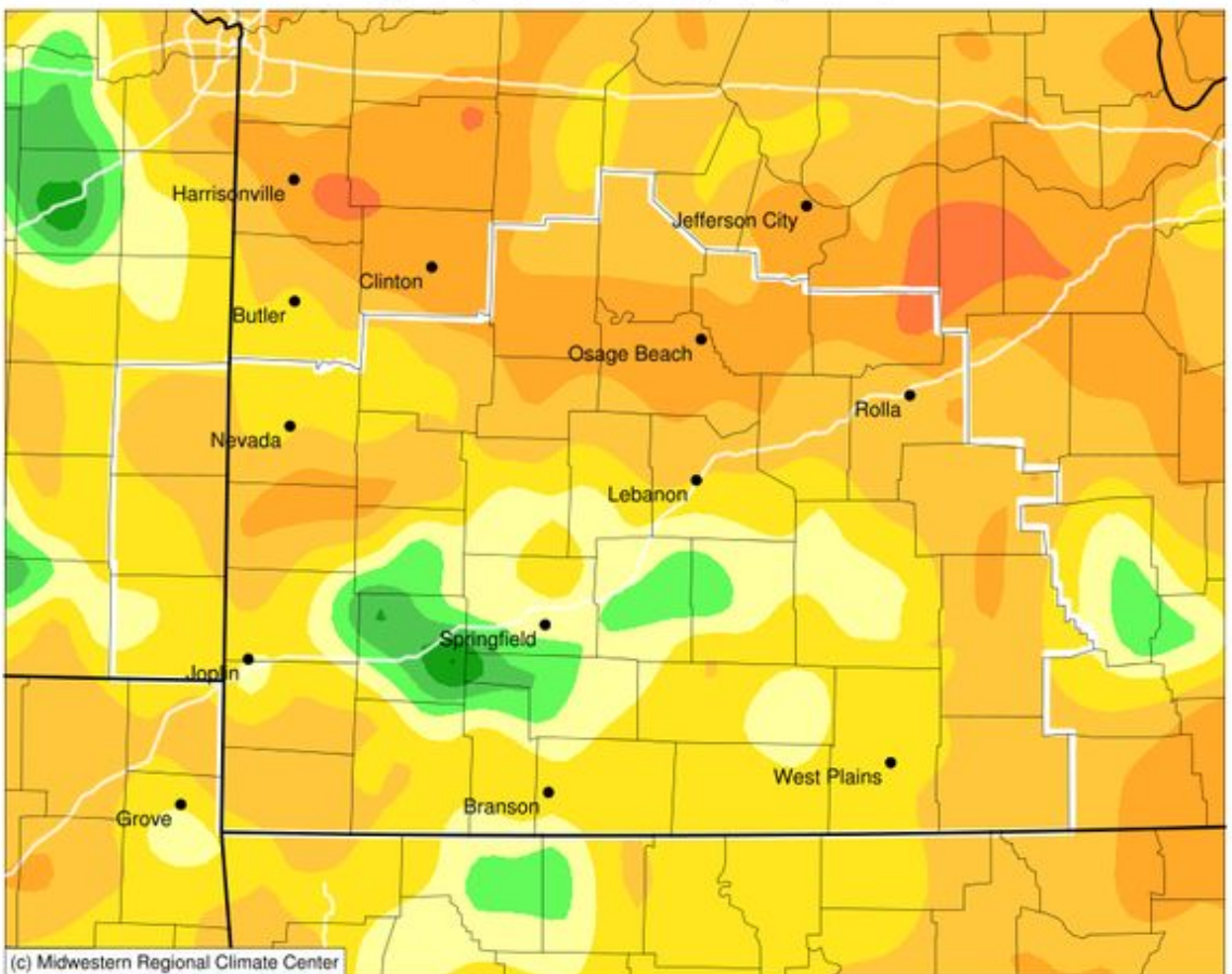
Accumulated Precipitation (in): Departure from 1991-2020 Normals May 01, 2023 to May 31, 2023
