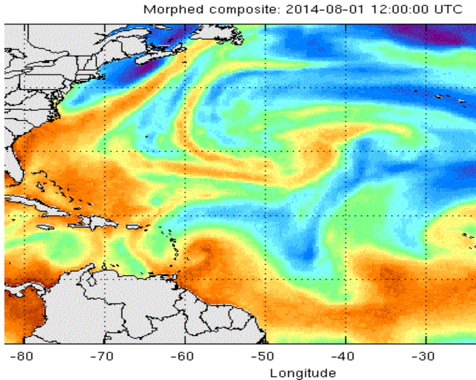
Figure 3. Morphed integrated microwave image (total precipitable water) from the Cooperative Institute for Meteorological Satellite Studies (CIMSS), August 1, 2014 for 1200 UTC.
