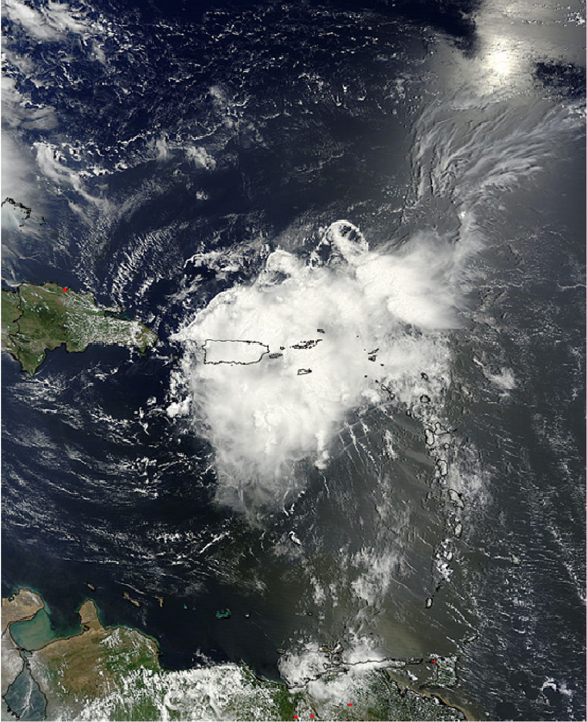
Figure 9. True color MODIS satellite image as Bertha was moving over Puerto Rico and the Virgin Islands. The center was 55 miles south of Ponce.
