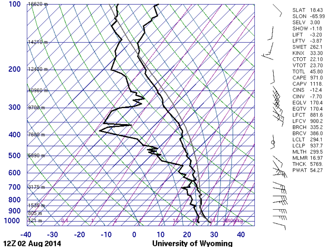
Figure 7. Upper air sounding for San Juan International Airport (TJSJ) at 1200 UTC August 2, 2014.
