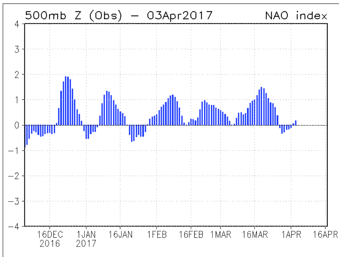
Figure 21: Observed standardized values of the daily NAO since December 2016. The NAO has generally been positive over the past several months with strong positive anomalies predominating in March.
