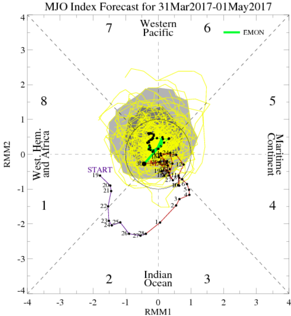
Figure 15: Monthly forecast of the MJO from the ECMWF model. The ECMWF model calls for continued weak MJO activity, as indicated by the green line being near the center of the circle.
