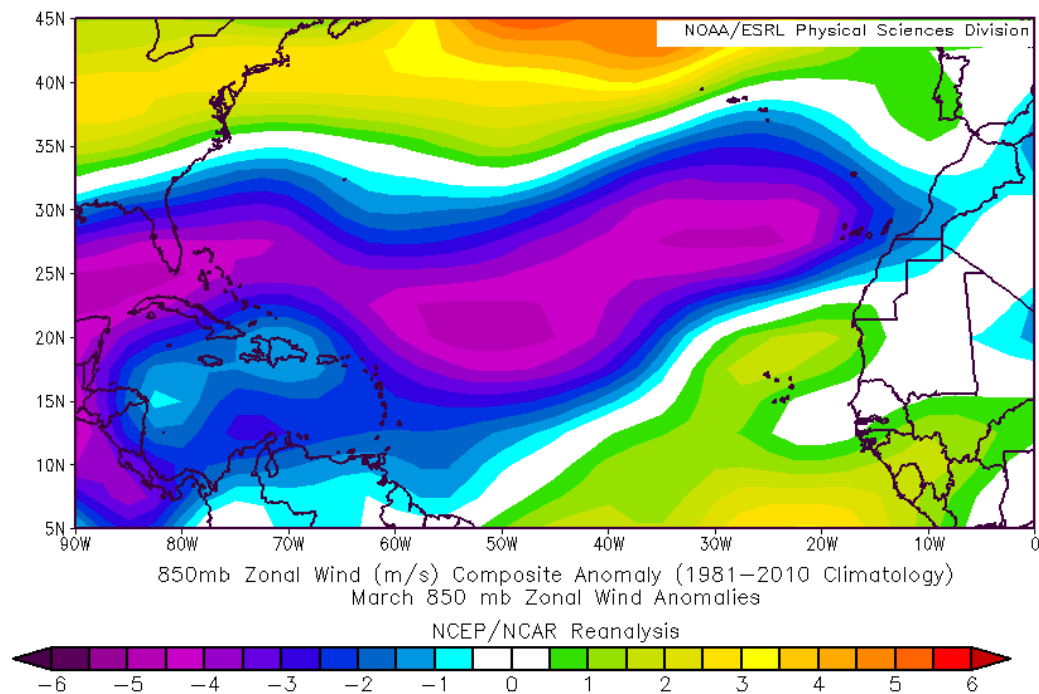
Figure 22: March low-level wind anomalies across the tropical and subtropical Atlantic. In general, easterly wind anomalies have prevailed, indicative of stronger than normal trade winds.
