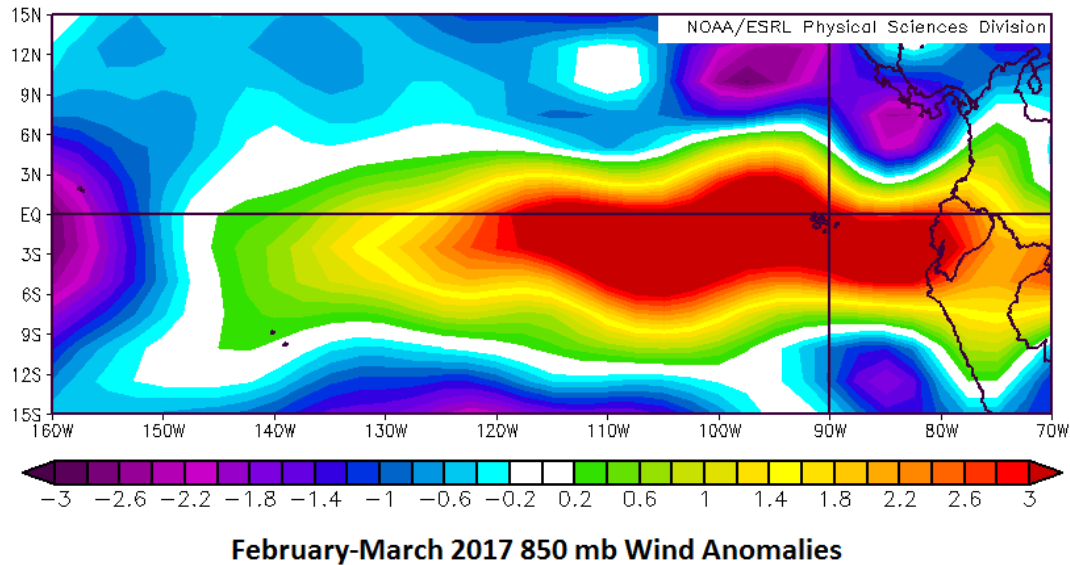
Figure 12: February through March 2017 850 mb zonal wind anomalies across the tropical eastern and central Pacific. The trade winds have been much weaker than normal across the eastern part of the basin.
