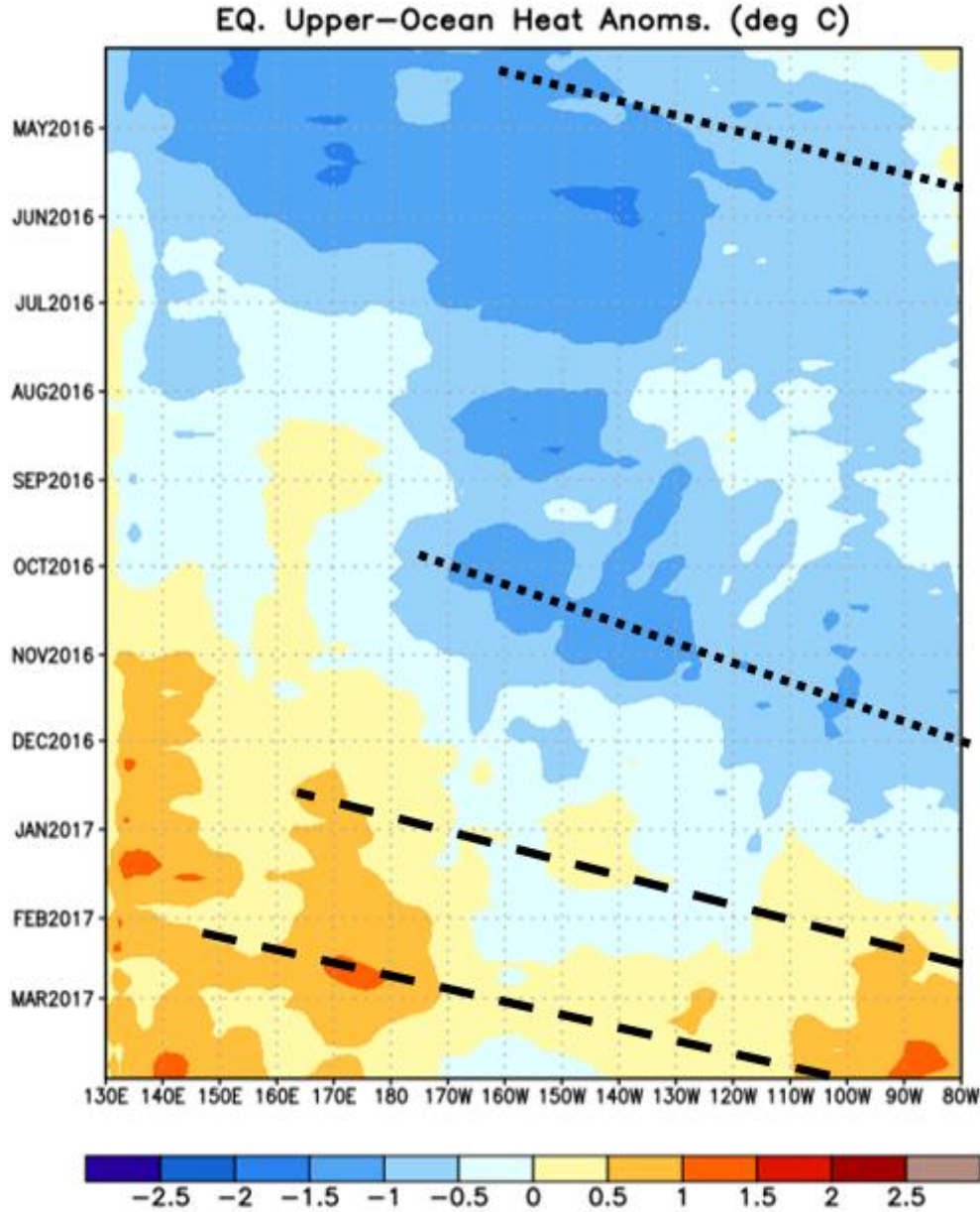
Figure 11: Upper-ocean heat content anomalies in the tropical Pacific since April 2016. Dashed lines indicate downwelling Kelvin waves, while dotted lines indicate upwelling Kelvin waves. Downwelling Kelvin waves result in upper-ocean heat content increases, while upwelling Kelvin waves result in upper-ocean heat content decreases.
