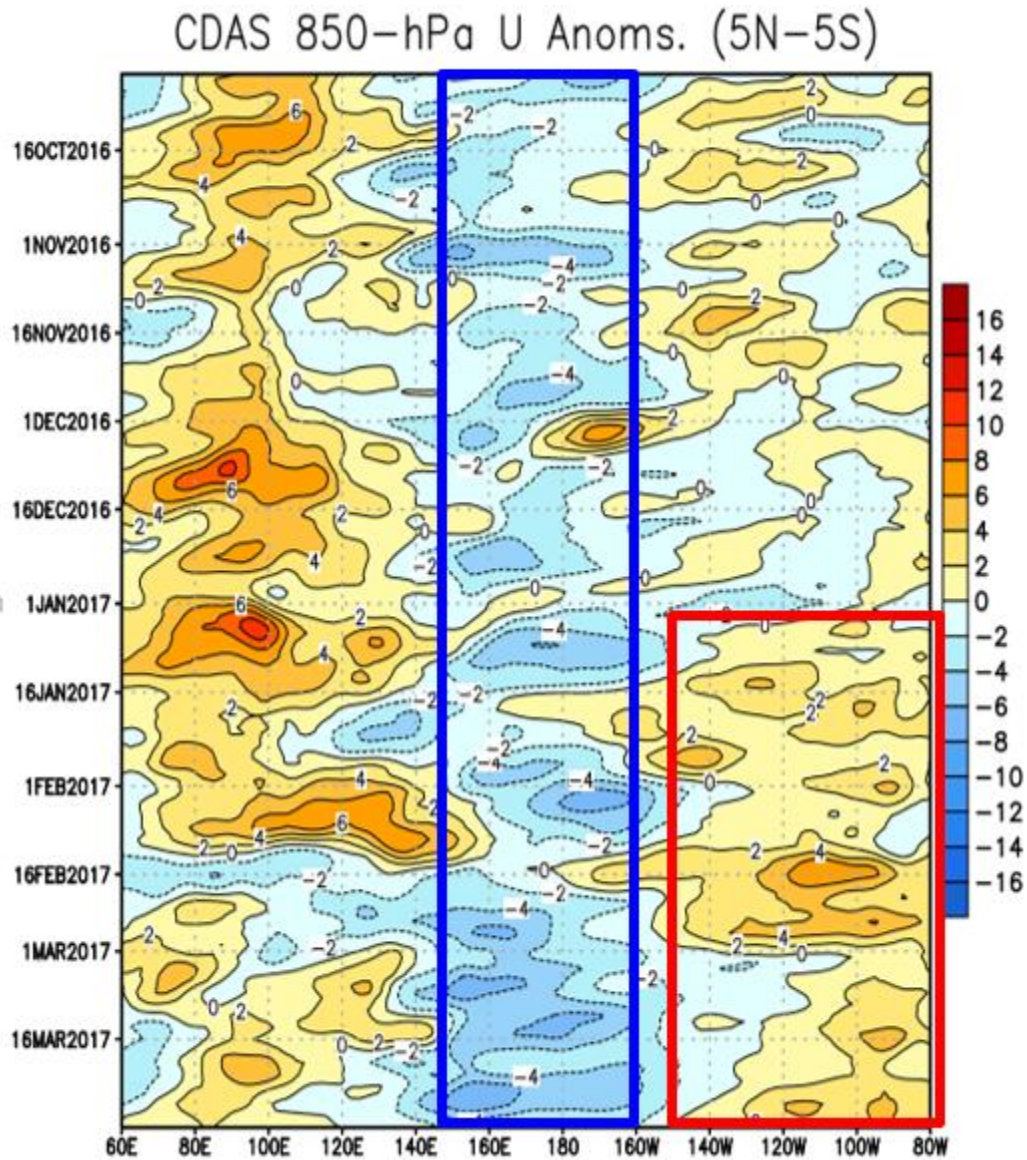
Figure 13: Low-level wind anomalies across the tropical Pacific since October 2016.
