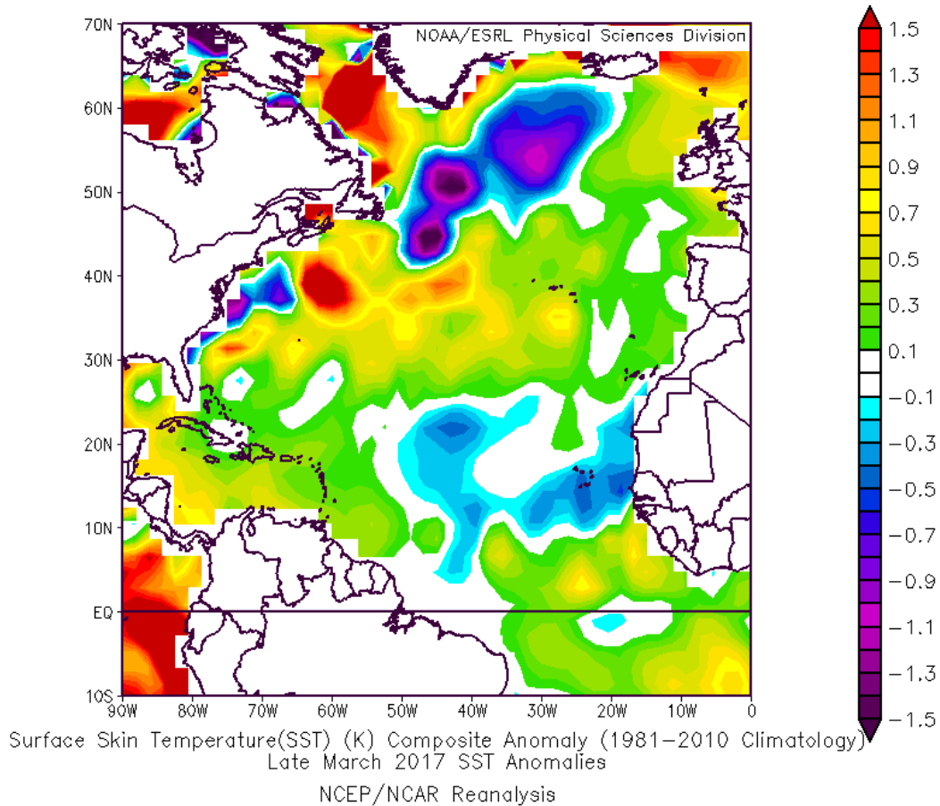
Figure 19: Late March 2017 SST anomaly pattern across the Atlantic Ocean.
