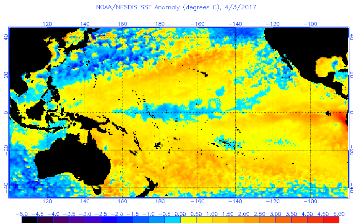
Figure 10: Current SST anomalies across the tropical and subtropical Pacific. Note the very warm SST anomalies that currently exist off of the west coast of South America.
