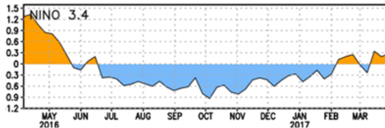
Figure 8: Nino 3.4 SST anomalies from April 2016 through March 2017. Figure courtesy of Climate Prediction Center.
