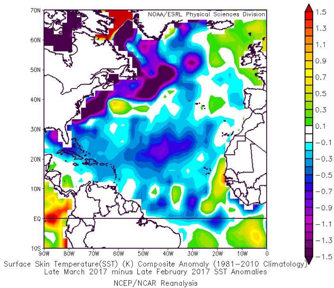
Figure 20: Late March 2017 minus late February 2017 SST anomalies. Most of the North Atlantic has undergone anomalous cooling.
