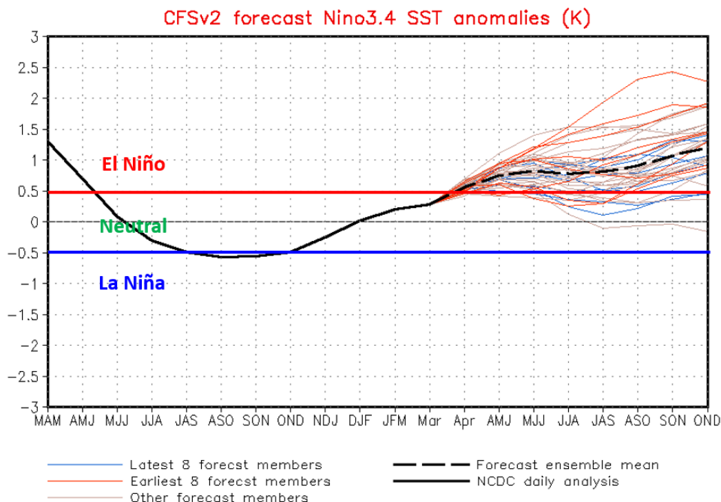
Figure 18: A recent forecast from the CFSv2 model, with the ensemble mean calling for borderline weak/moderate El Niño conditions for the late summer/early fall.
