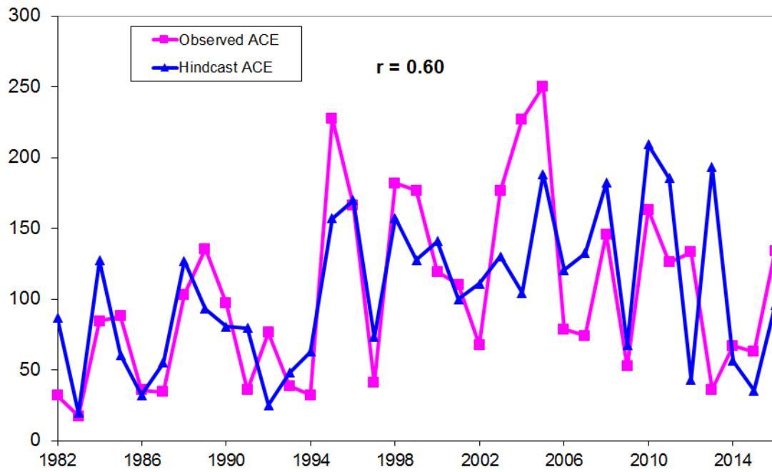
Figure 1: Observed versus early April hindcast values of ACE for 1982-2010 along with real-time forecast values for 2011-2016.
