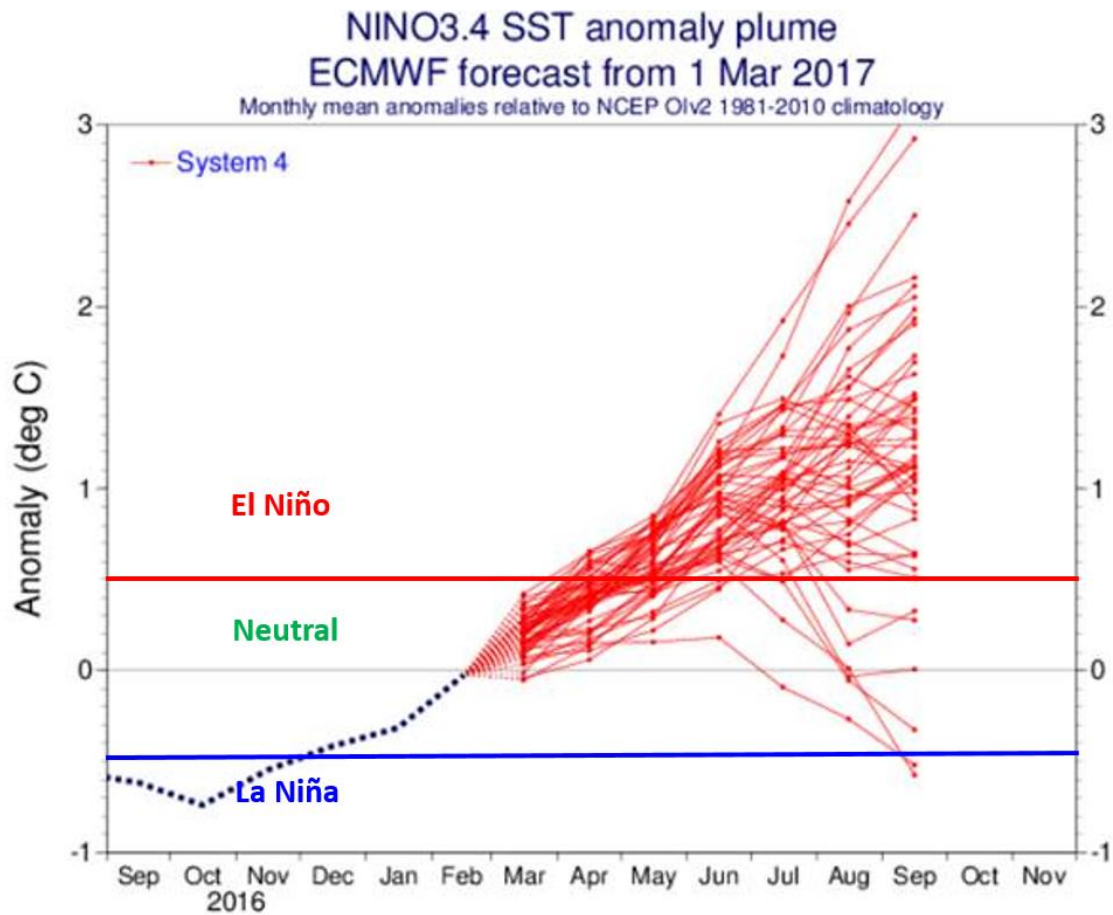
Figure 17: ECMWF ensemble model forecast for the Nino 3.4 region. Most members are calling for El Niño conditions by September, but there is large spread at this long lead time.
