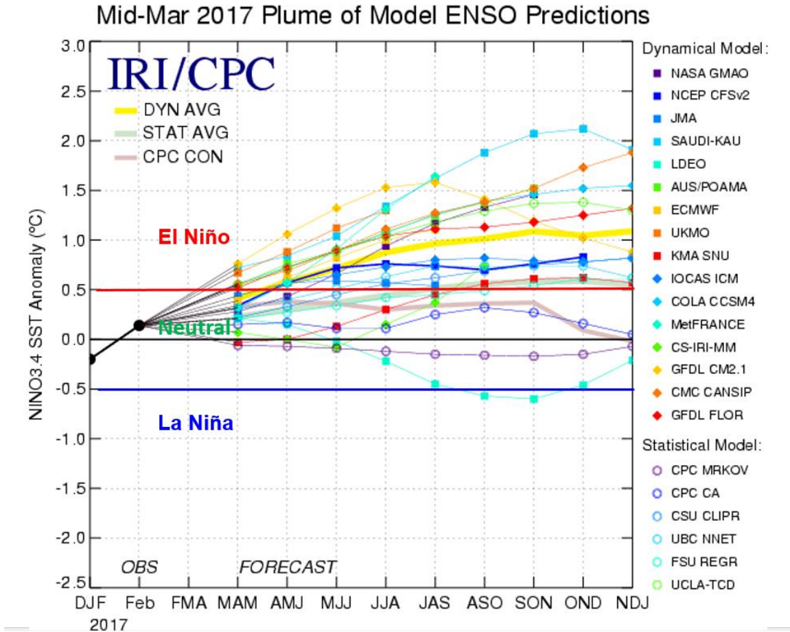
Figure 16: ENSO forecasts from various statistical and dynamical models for the Nino 3.4 SST anomaly based on March initial conditions. Figure courtesy of the International Research Institute (IRI). Most dynamical models are calling for El Niño during August-October.
