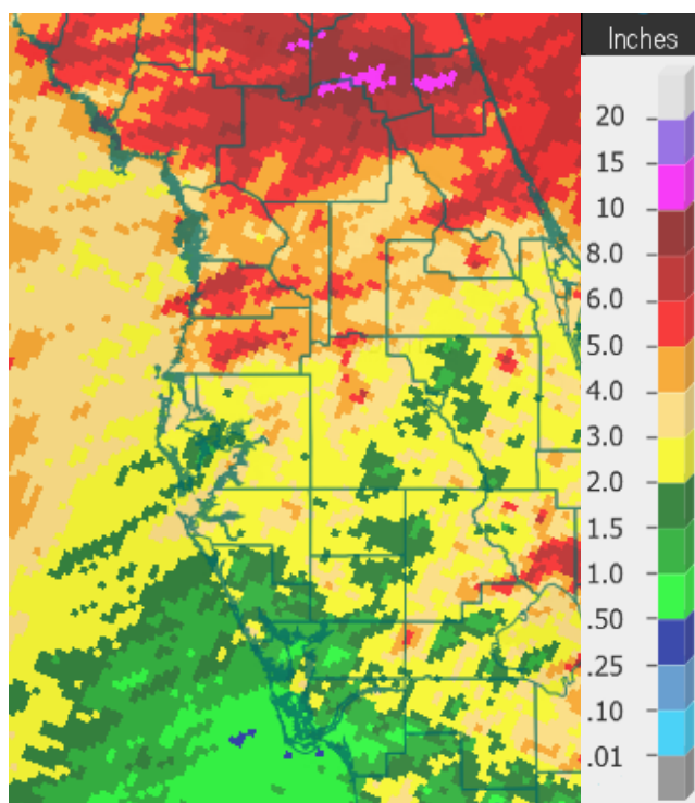
April 2018 Rainfall
