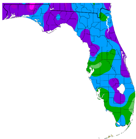
Temperature (F) 6/1/2025 – 8/31/2025
