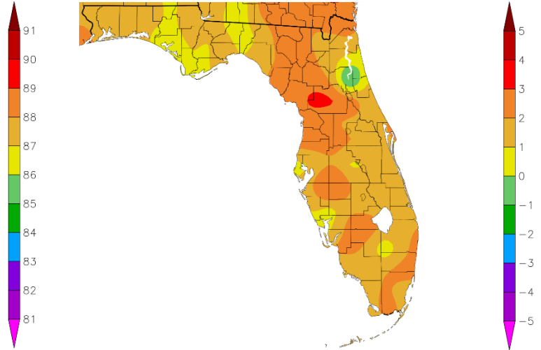
Departure from Normal Temperature (F) 7/1/2026 – 7/30/2026
