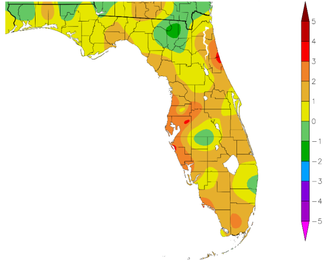
Departure from Normal Temperature (F) 7/1/2020 - 7/31/2020
