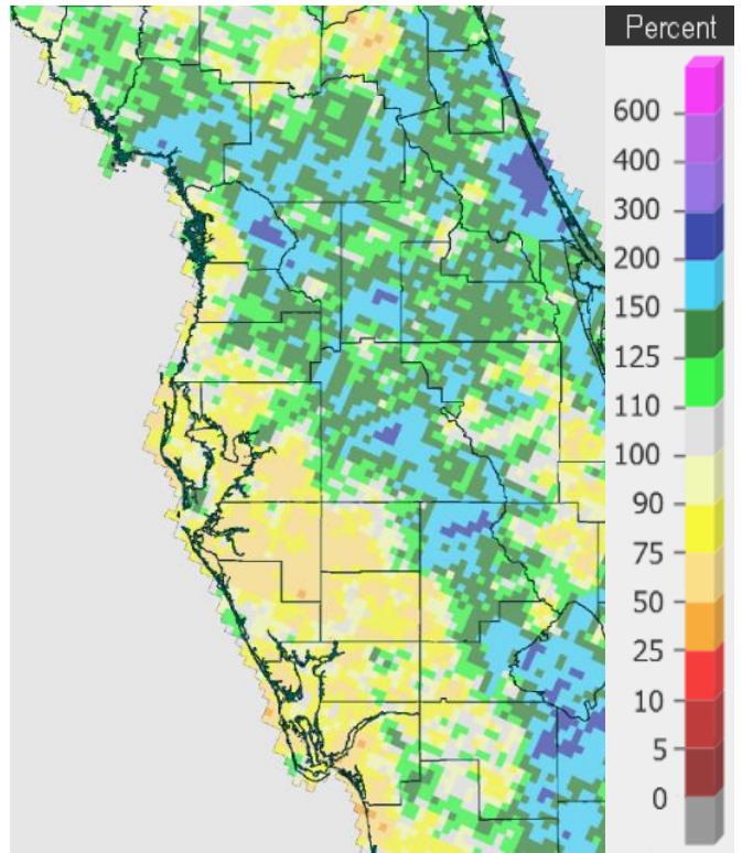
July 2020 Percent of Normal
