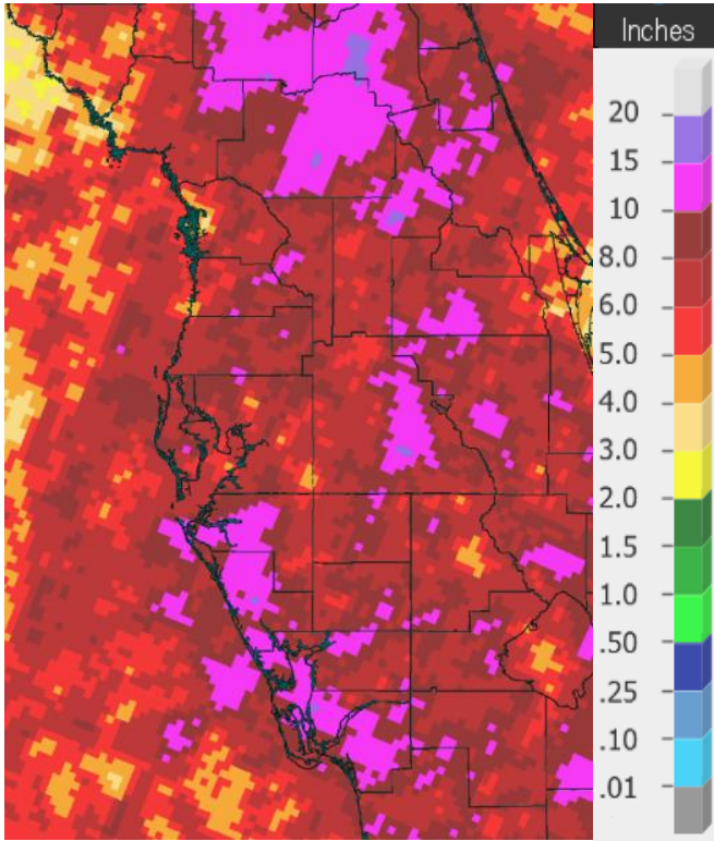
June 2020 Rainfall
