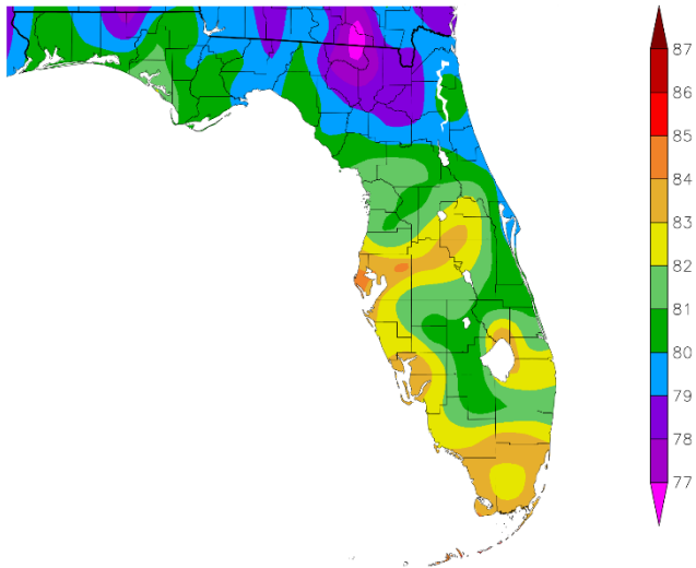
Temperature (F) 6/1/2020 - 6/30/2020
