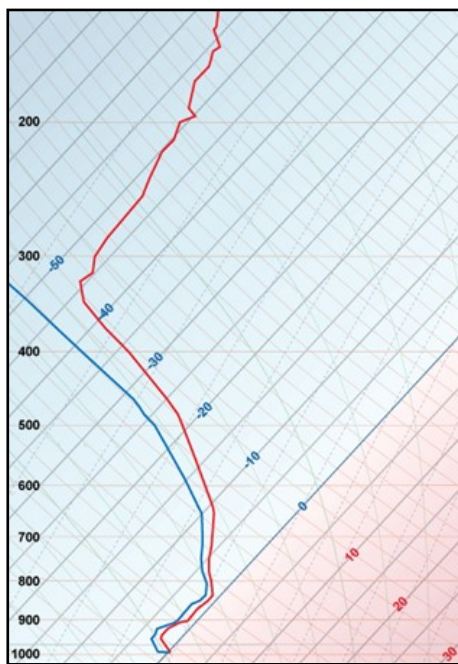
Figure 1. A typical “snow” sounding.
