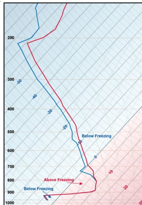
Figure 2. A typical “freezing rain” sounding.
