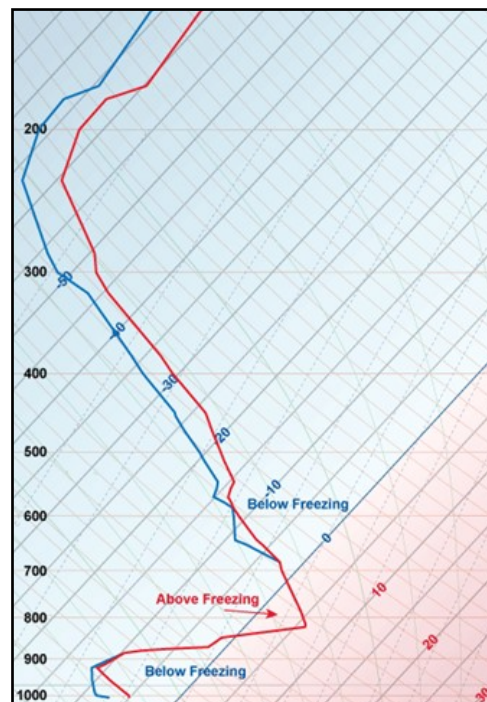
Figure 3: A typical “sleet” sounding.
