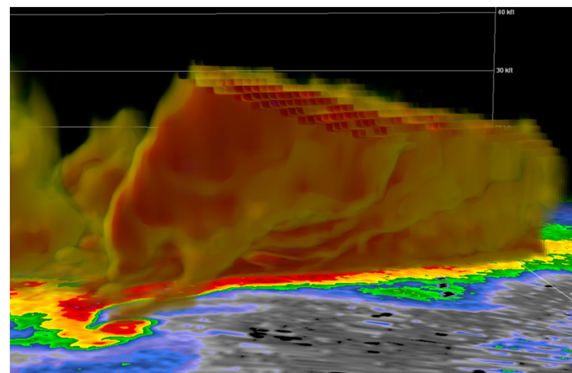
Tornadic Supercell near Tulsa, OK 3/30/16
