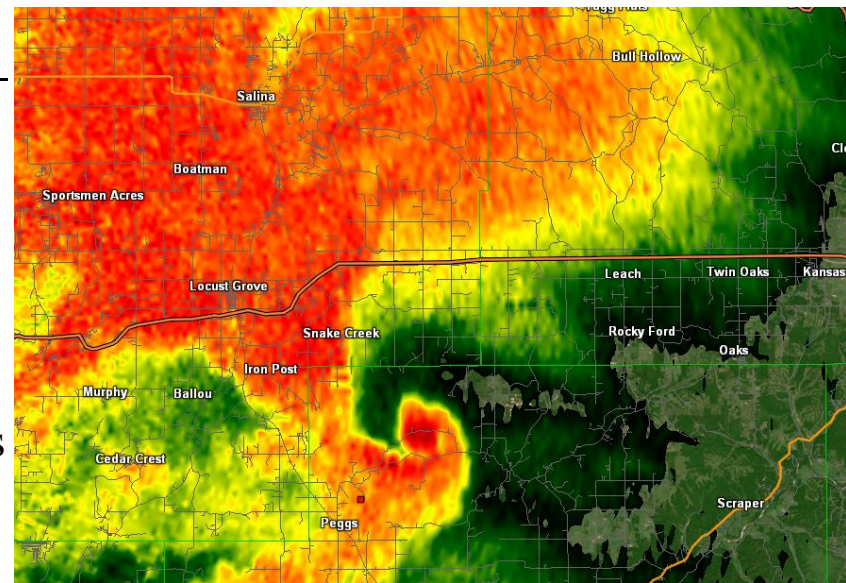
Tornadic Supercell near Peggs, OK 5/20/19
