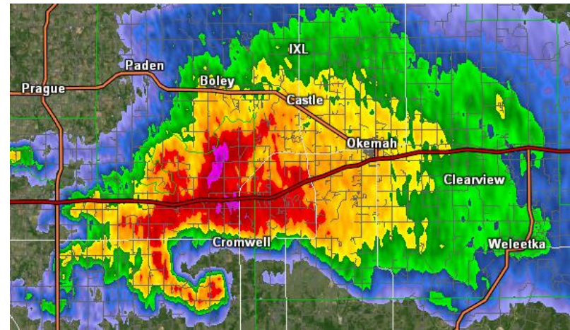
Cyclic Tornado Supercell, May 4, 2022
