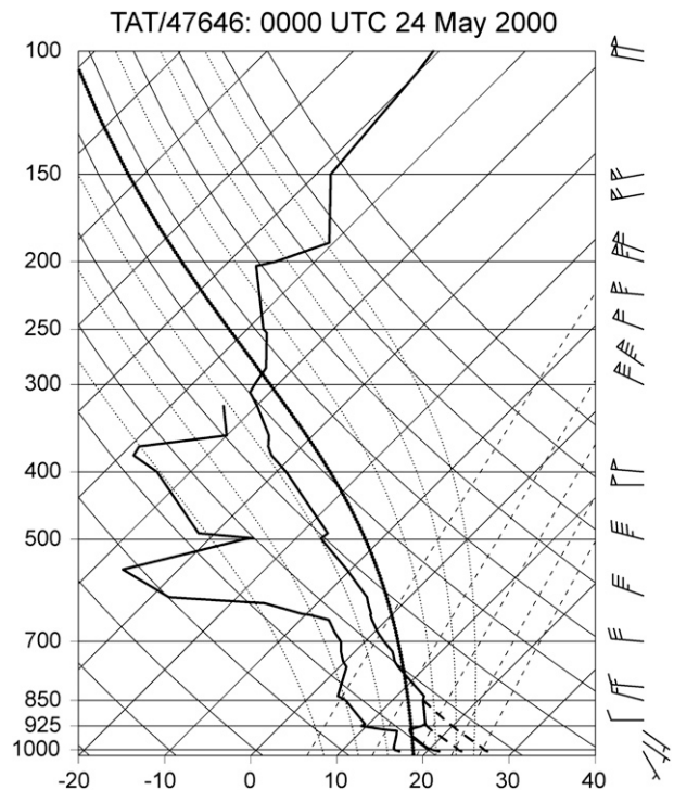
FIG. 2. Observed skew T - \log p sounding (thick solid lines) for Tateno, Japan, valid at 0000 UTC (0900 JST) 24 May 2000. Half, whole, and flag wind barbs denote 2.5, 5, and 25 \text{ m s}^{-1} , respectively. Temperature is given along the abscissa ( ^{\circ}\text{C} ) and pressure is plotted along the ordinate (hPa). The two thick dashed lines in the boundary layer represent modified temperature profiles for observed surface conditions and dry adiabatic lapse rates at Koga ( 24^{\circ}\text{C} , 1120 JST) and Sakura ( 27^{\circ}\text{C} , 1210 JST) just prior to passage of the Kanto Plain supercell (as given in S08). The moist adiabat for the Sakura mixed-layer parcel is also highlighted by the thick dotted line. Refer to Table 2 for variables calculated from these profiles.
