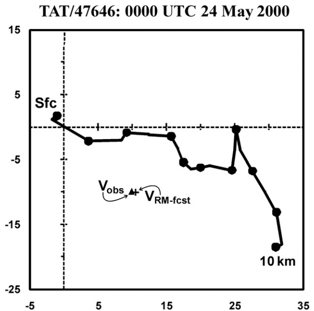
FIG. 1. Observed 0–10-km hodograph ( \text{m s}^{-1} ) for Tateno, Japan, valid at 0000 UTC 24 May 2000. Wind data are plotted every 500 m AGL, but markers (filled circles) are given only at 1-km intervals. Here, \mathbf{V}_{\text{obs}} (filled triangle) represents the observed supercell motion and \mathbf{V}_{\text{RM-fcst}} (plus sign) represents the predicted right-moving supercell motion as computed in Bunkers et al. (2000). Refer to Table 2 for variables calculated from this hodograph.
