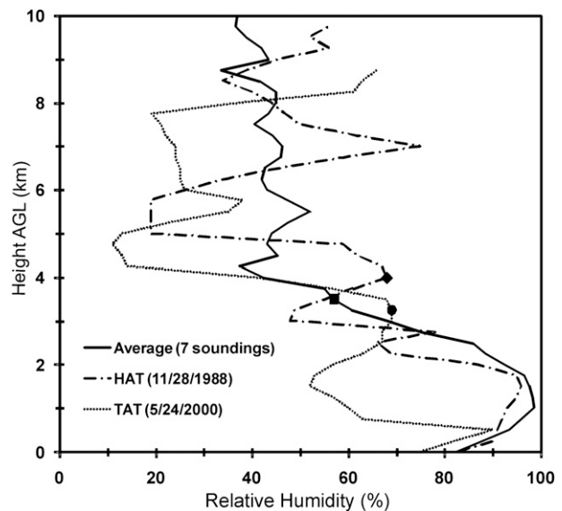
FIG. 3. Plot of RH as a function of height AGL for (solid line) the average of the seven soundings listed at the top of Table 3, (dashed-dotted line) the Cape Hatteras, NC (HAT), sounding from 1200 UTC 28 Nov 1988 [i.e., indicative of the Raleigh, NC, tornadic environment; see Kulie and Lin (1998)], and (dashed line) the unmodified TAT sounding in Fig. 2. The markers indicate the height of the melting level for each of the three RH profiles. Refer to section 4 for the corresponding discussion.
