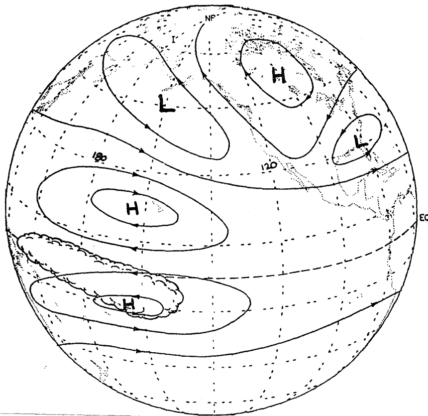
Figure 2. Schematic of upper tropospheric height anomalies following the peak of a typical ENSO episode. Cloud outline indicates region of enhanced precipitation (after Horel and Wallace, 1981).
