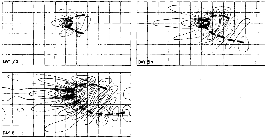
Figure 1. The vorticity perturbation generated with a circular forcing centered on 30 N. Heavy dashed lines indicate wave trains (after Hoskins, et al , 1977).
