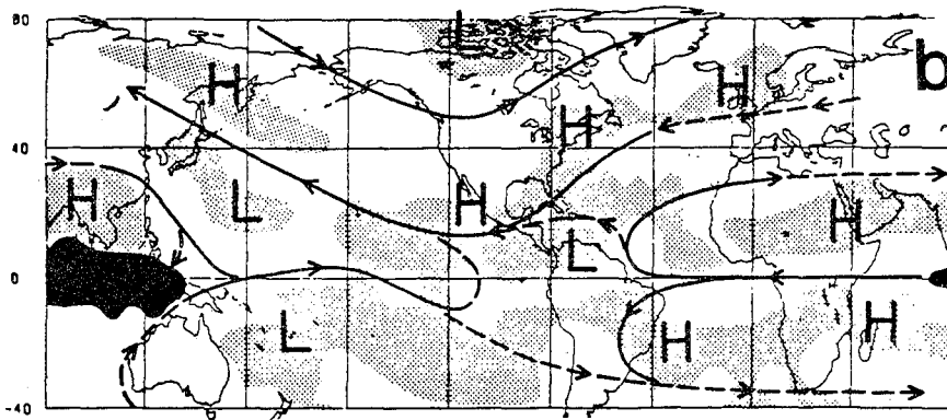
Figure 6. Schematic representation of cross-spectral coherence and phase information between outgoing longwave radiation and 250 mb streamfunction for cloudiness centered at EQ, 100 E (after Weickmann, et al, 1985). Dark shading represents the anomalous cloudiness. Light shading represents the location where the cross-spectral coherence is significant at 95%.
