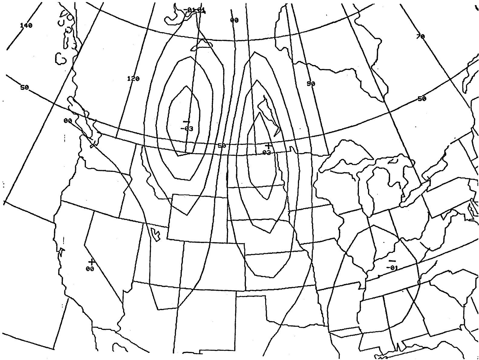
Fig. 5 Diagnosed vertical motion applying Q-vector analysis to model forecast data valid for 00Z, October 22, 1987.
