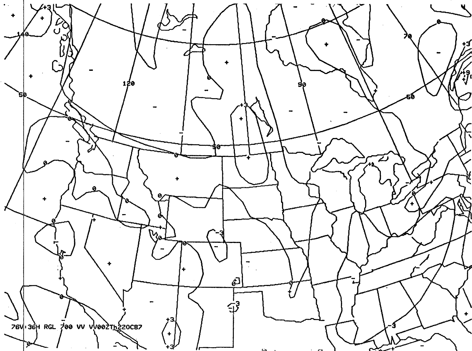
Fig. 4 The 36-hour NGM vertical motion forecast valid 00Z, October 22, 1987.
