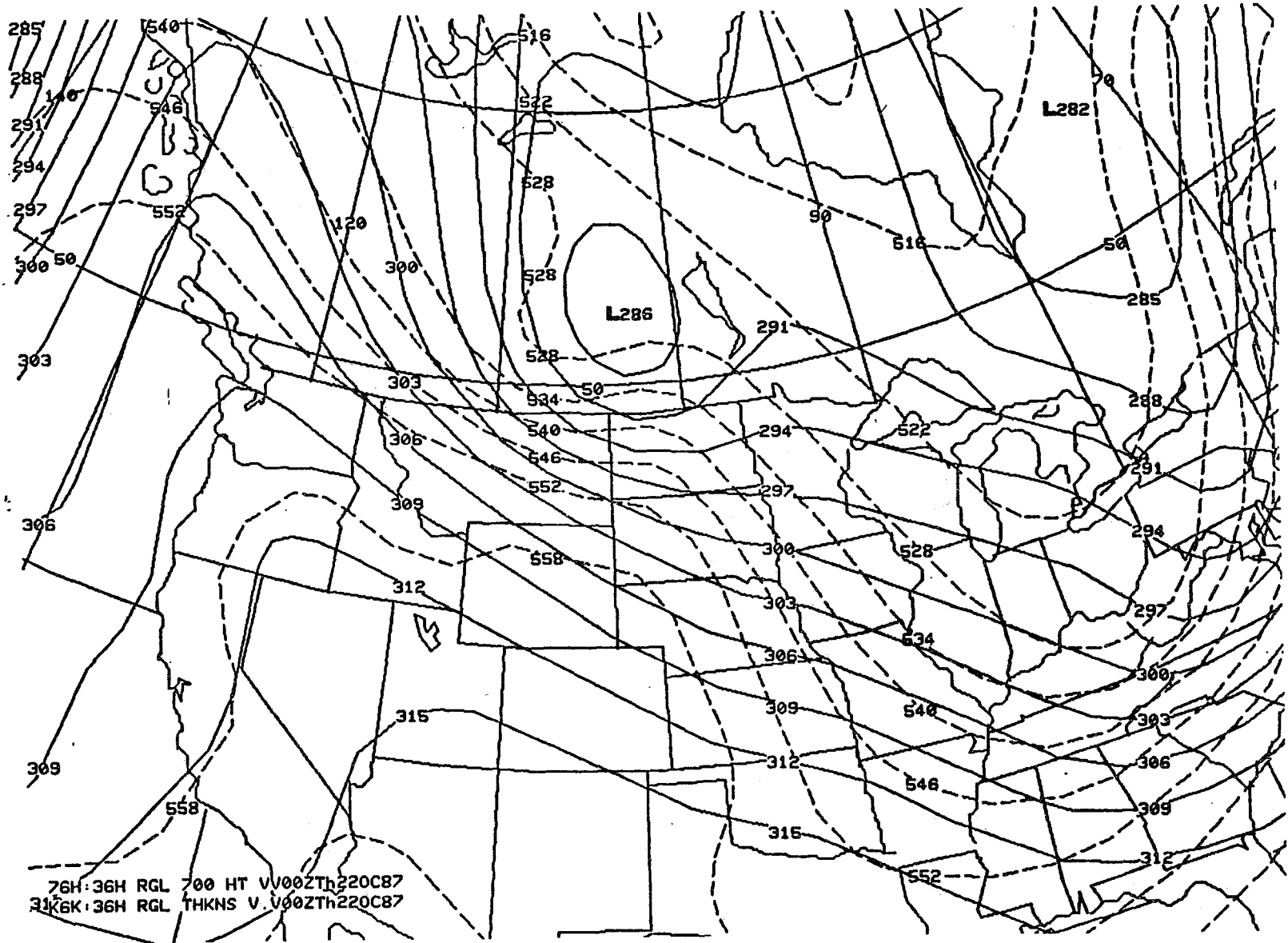
Fig. 3 The 36-hour NCM forecast for 700 mb heights (solid) and thickness (dashed) valid 00Z, October 22, 1987.
